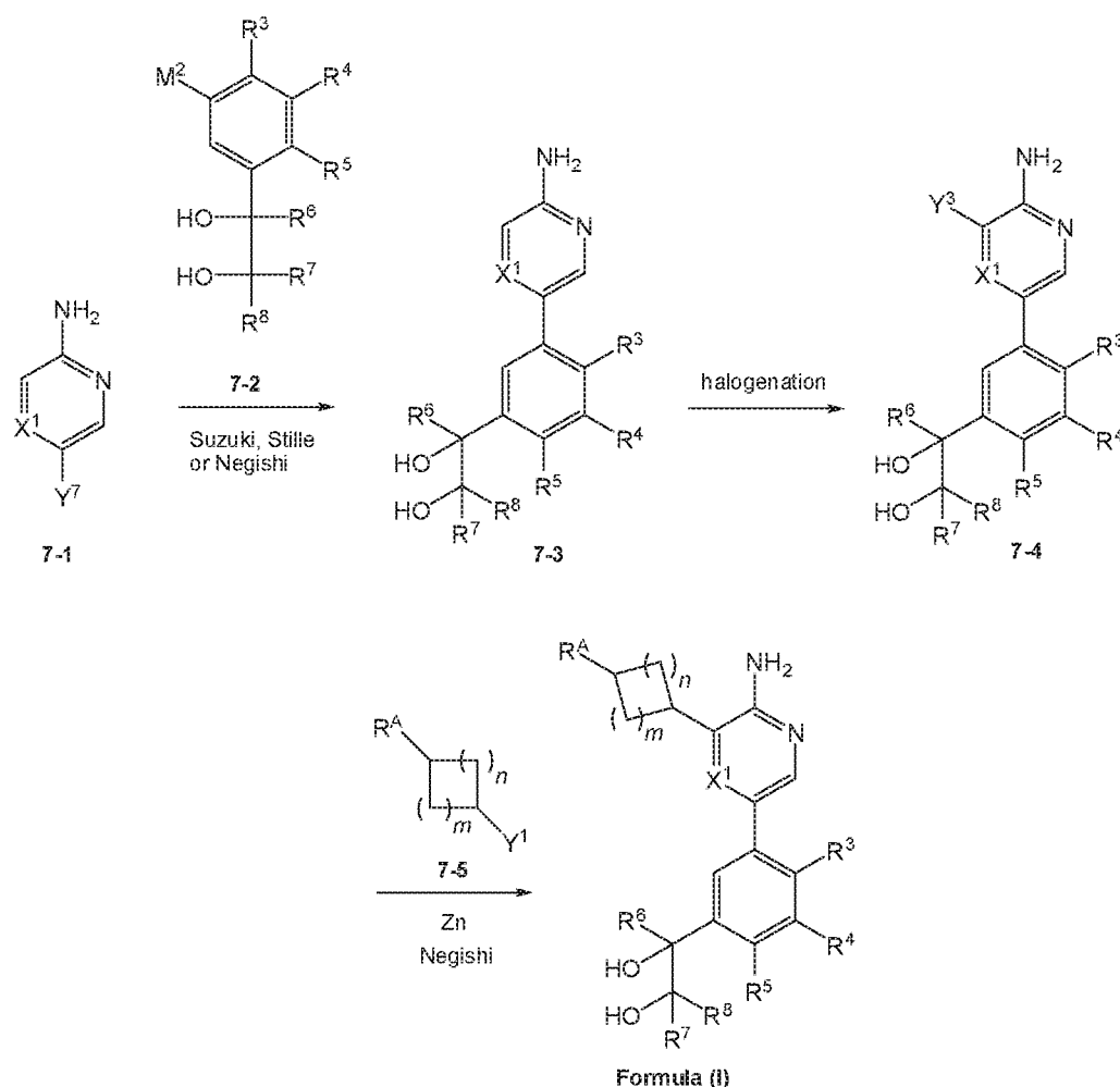
Scheme 7.
