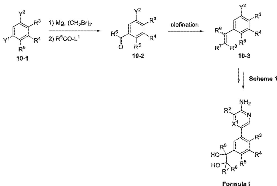
Scheme 10.
