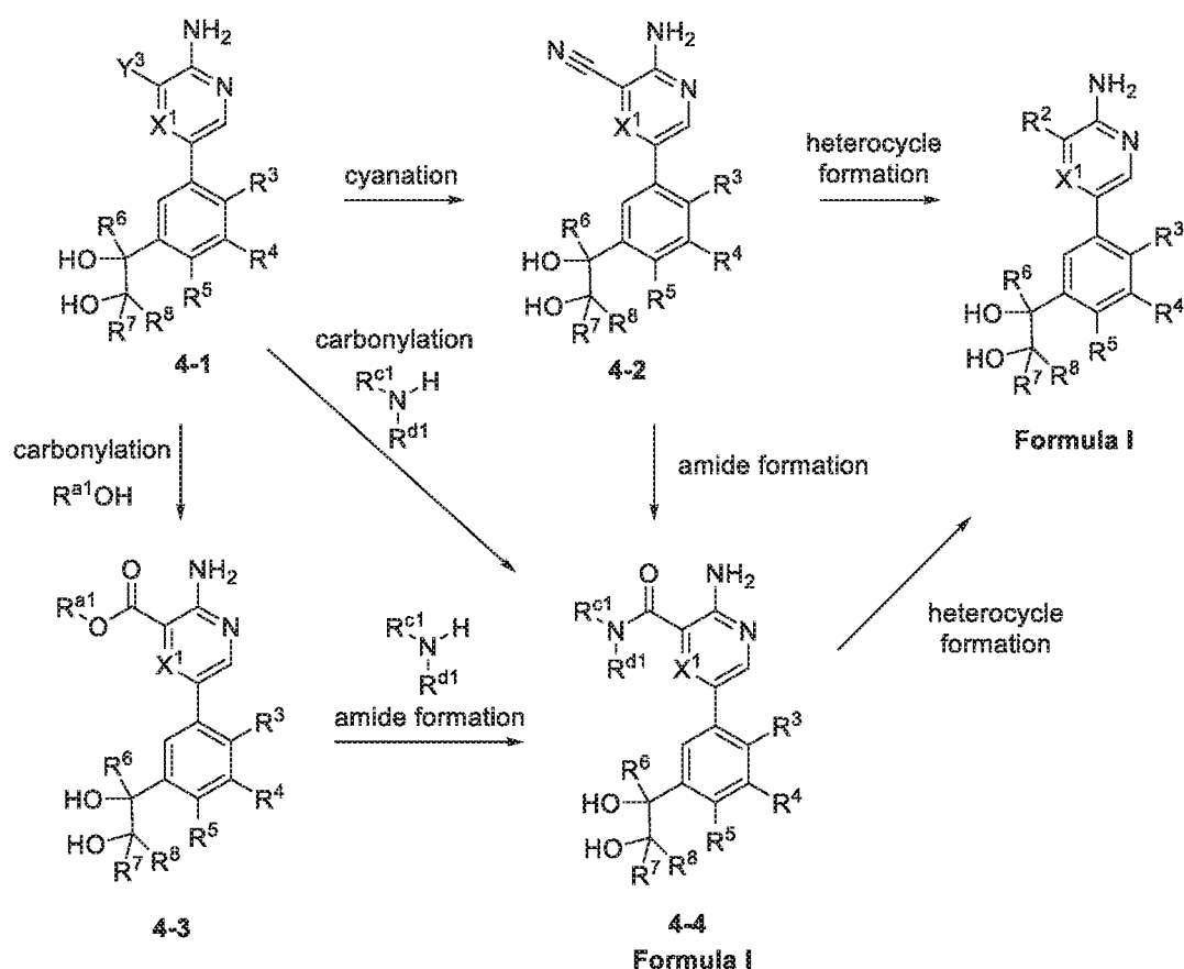
Scheme 4.
