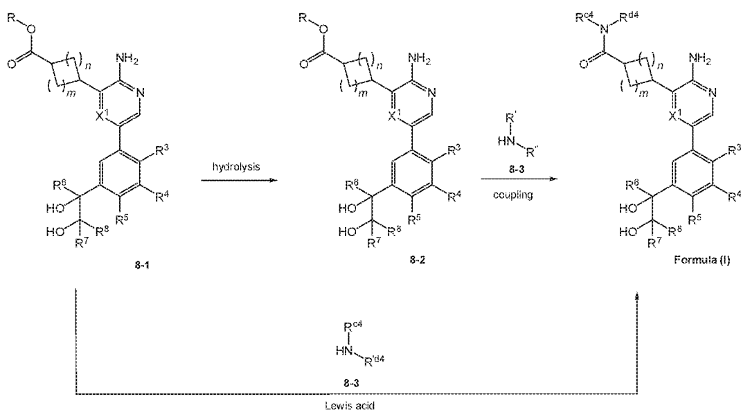
Scheme 8.
