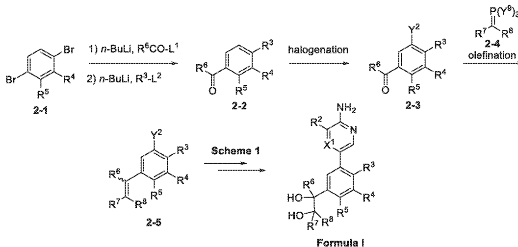
Scheme 2.
