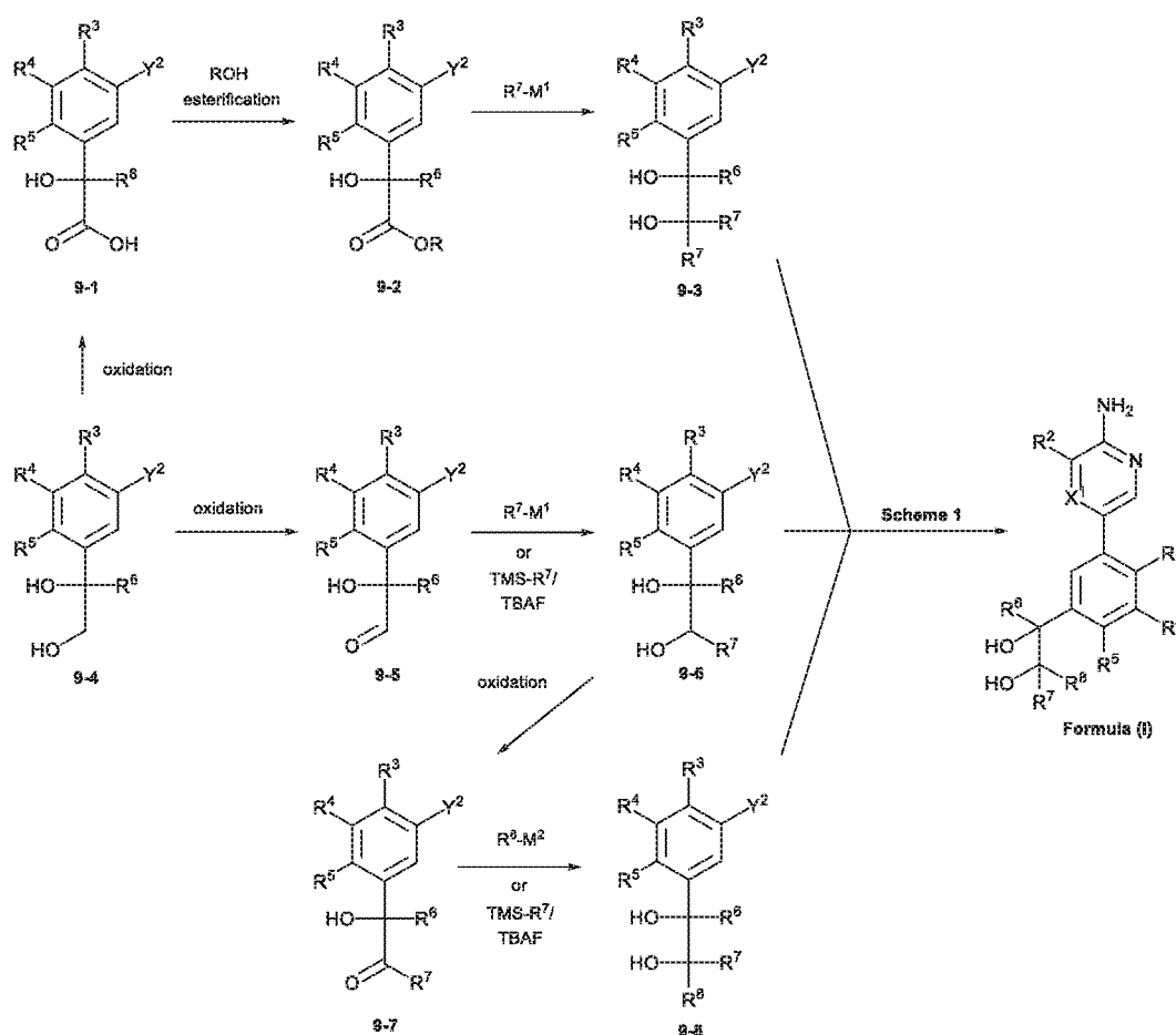
Scheme 9.
