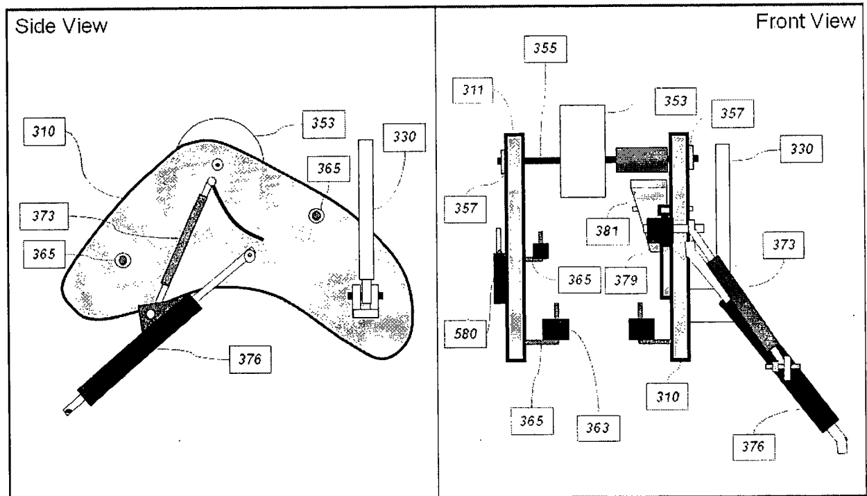
Figure 8: depicts the Safety & Handle System (300).
