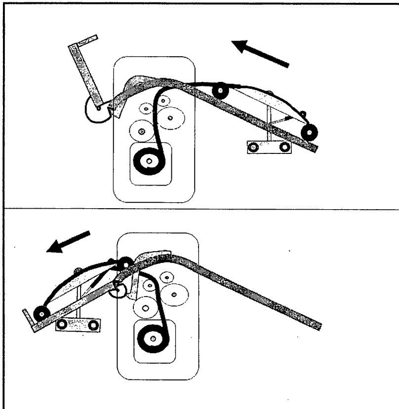
Figure 20: depicts how the Cable Drive System (400), the Car (200) and the Extender Arm (610) would interact.
