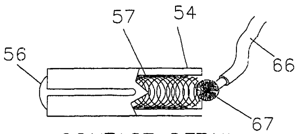
CONTACT DETAIL FIG. 14
