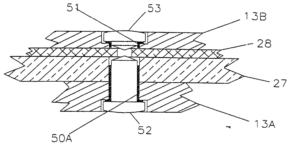
SECTION A-A FIGURE 6
