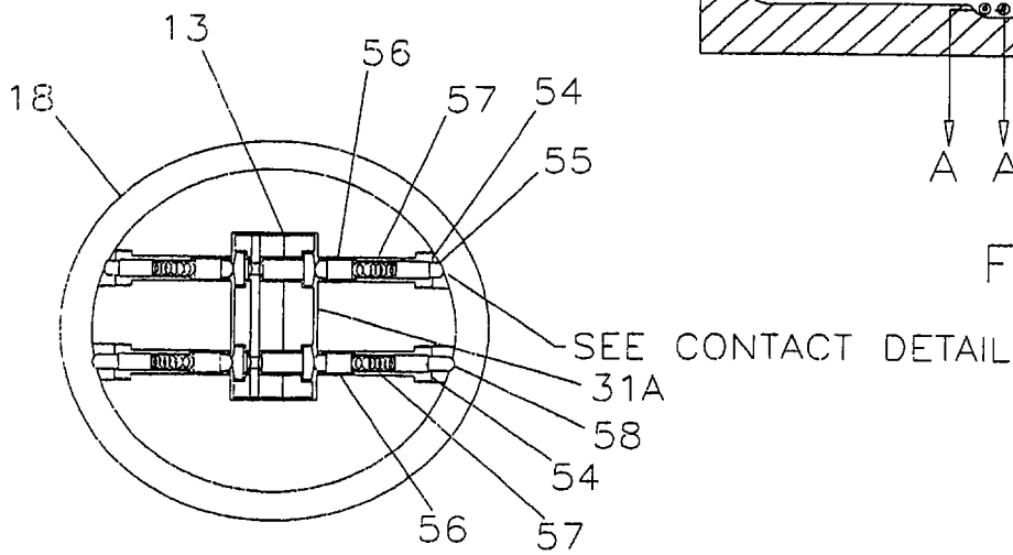
SECTION B-B FIGURE 7
