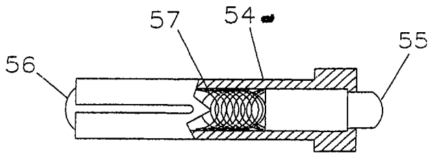
CONTACT DETAIL FIGURE 8
