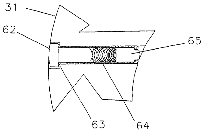
CONTACT DETAIL FIGURE 10
