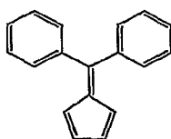
6,6-diphenylpentafulvene
