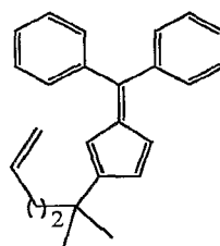
2-(1,1-dimethylpent-4-enyl)-6,6-diphenylpentafulvene
