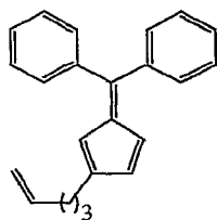
2-(pent-4-enyl)-6,6-diphenylpentafulvene
