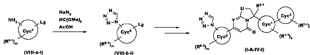
Reaction Scheme 12
