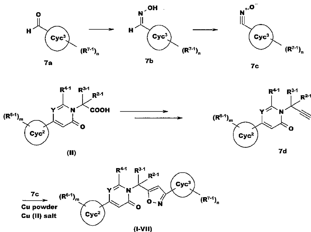
Reaction Scheme 7
