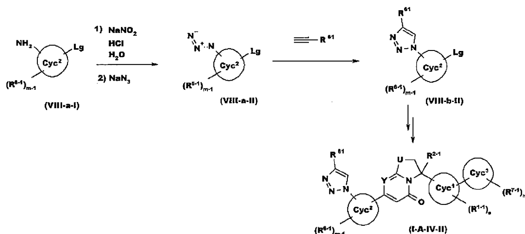
Reaction Scheme 13
