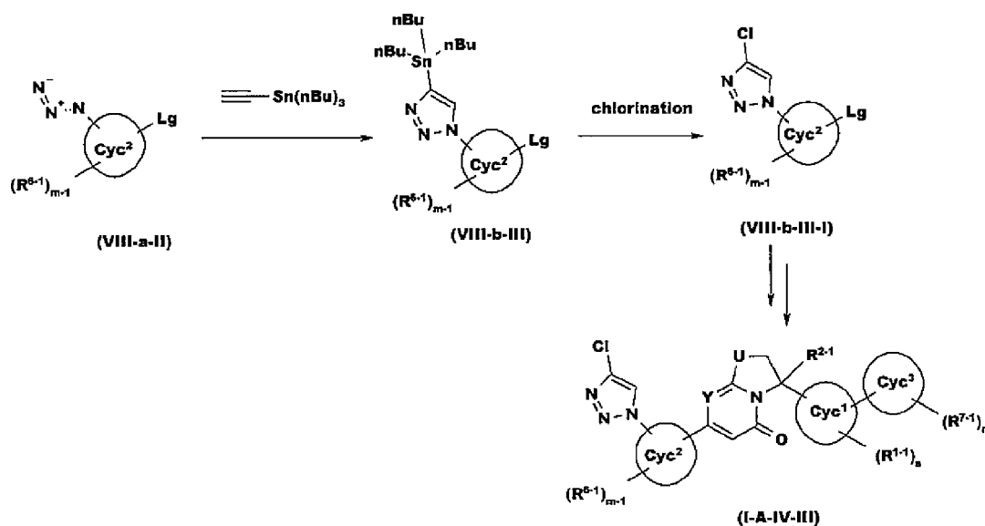
Reaction Scheme 14
