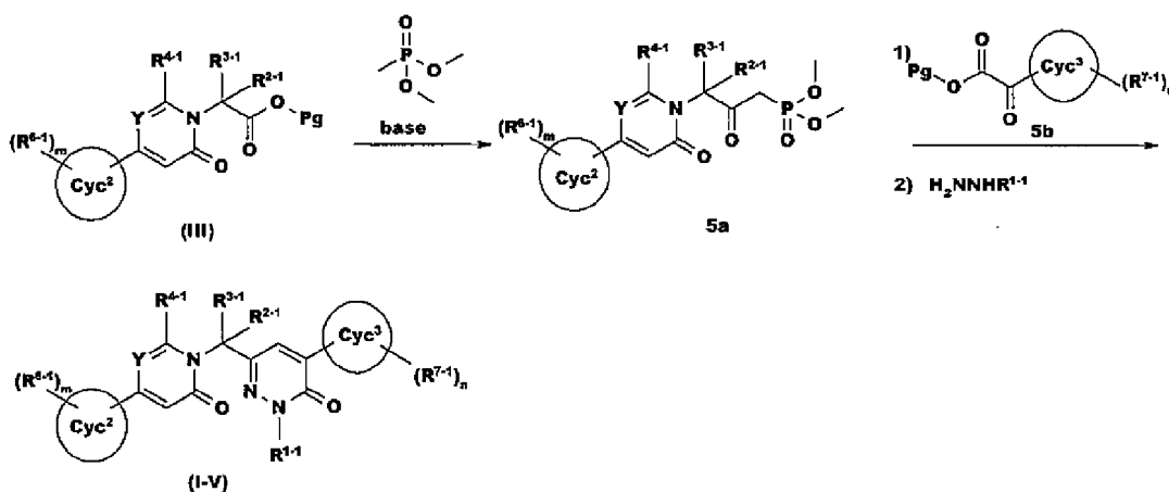
Reaction Scheme 5
