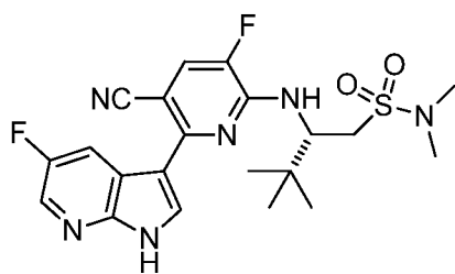
(S)-2-((5-Cyano-3-fluoro-6-((5-fluoro-1H-pyrrolo[2,3-b]pyridin-3-yl)pyridin-2-ylamino)-N,N,3,3-tetramethylbutane-1-sulfonamide (27)
