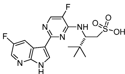
(S)-2-(5-fluoro-2-(5-fluoro-1H-pyrrolo[2,3-b]pyridin-3-yl)pyrimidin-4-ylamino)-3,3-dimethylbutane-1-sulfonic acid (11)
