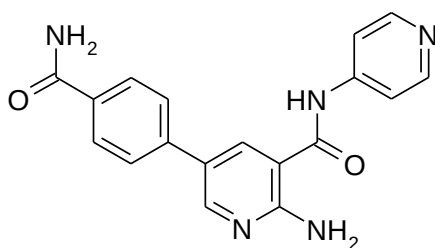
2-Amino-5-(4-carbamoyl-phenyl)-N-pyridin-4-yl-nicotinamide ("A88")
