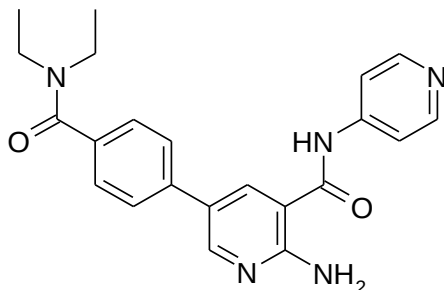
2-Amino-5-(4-diethylcarbamoyl-phenyl)-N-pyridin-4-yl-nicotinamide ("A87")
