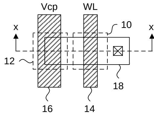
Figure 2 (Prior Art)
