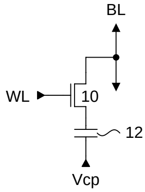
Figure 1 (Prior Art)
