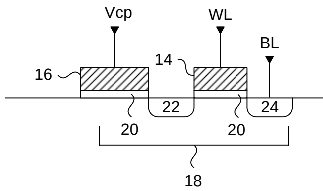
Figure 3 (Prior Art)
