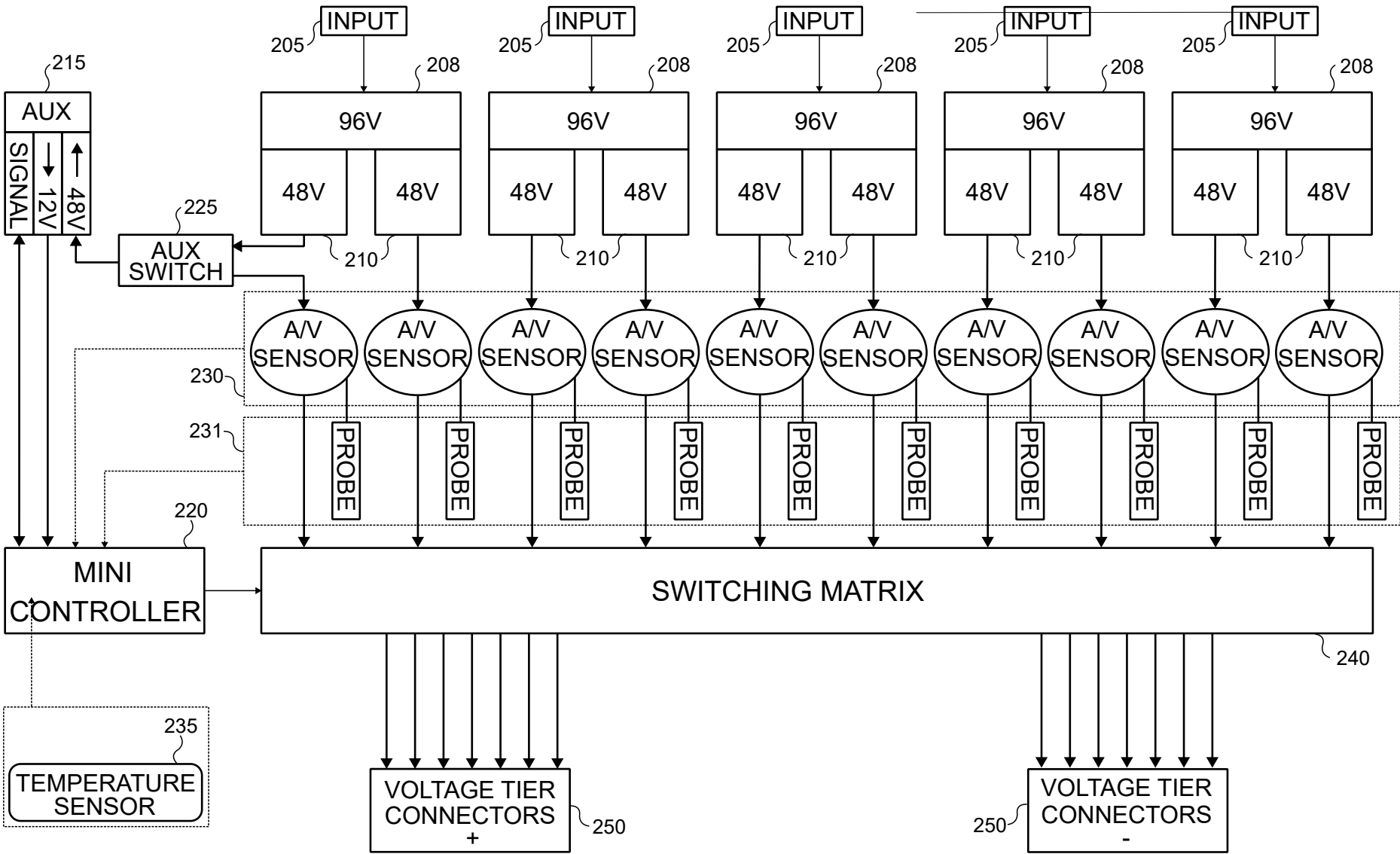
FIG. 4: POWER MODULE FUNCTIONAL BLOCK DIAGRAM
