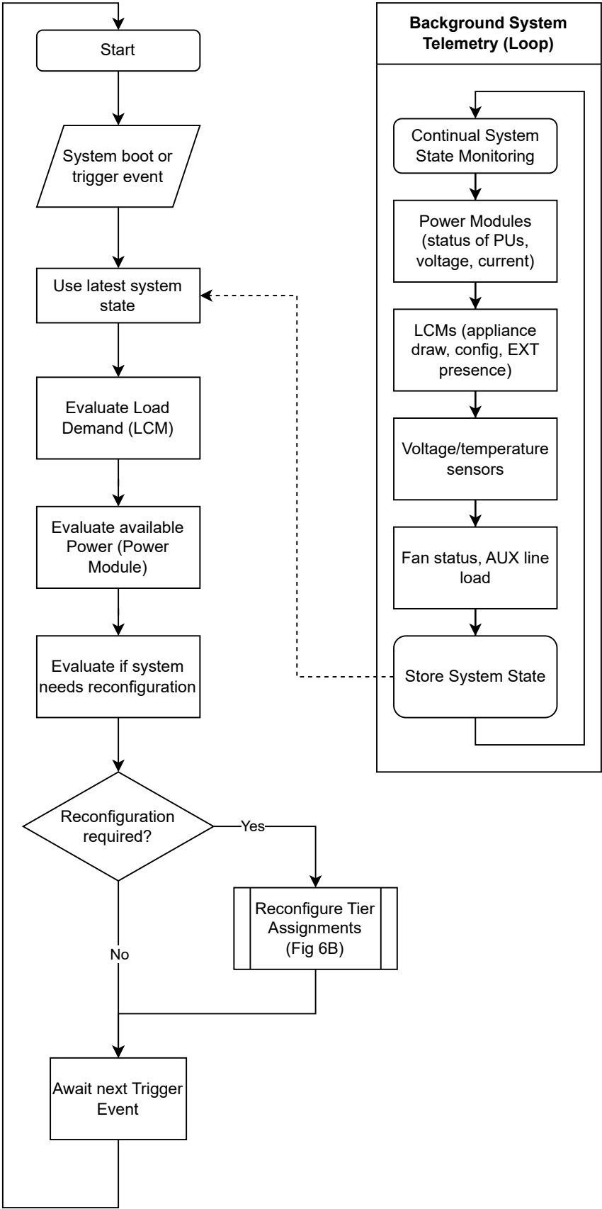
FIG. 6A: Main Logic Flowchart of Tier Assignment and Reconfiguration Process
