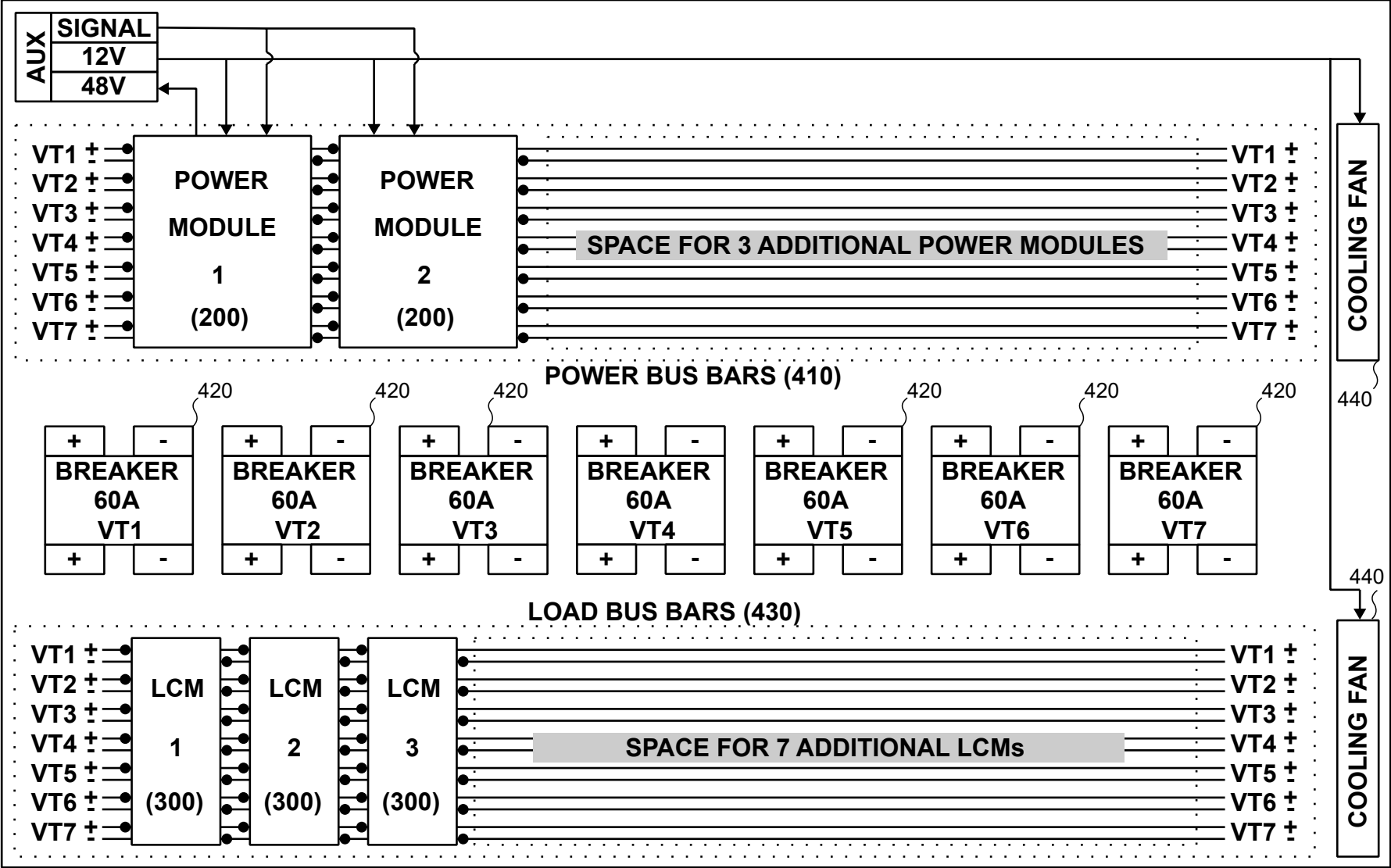
FIG 3: HIGH-VOLTAGE-DISTIBUTION-CASE (400)
