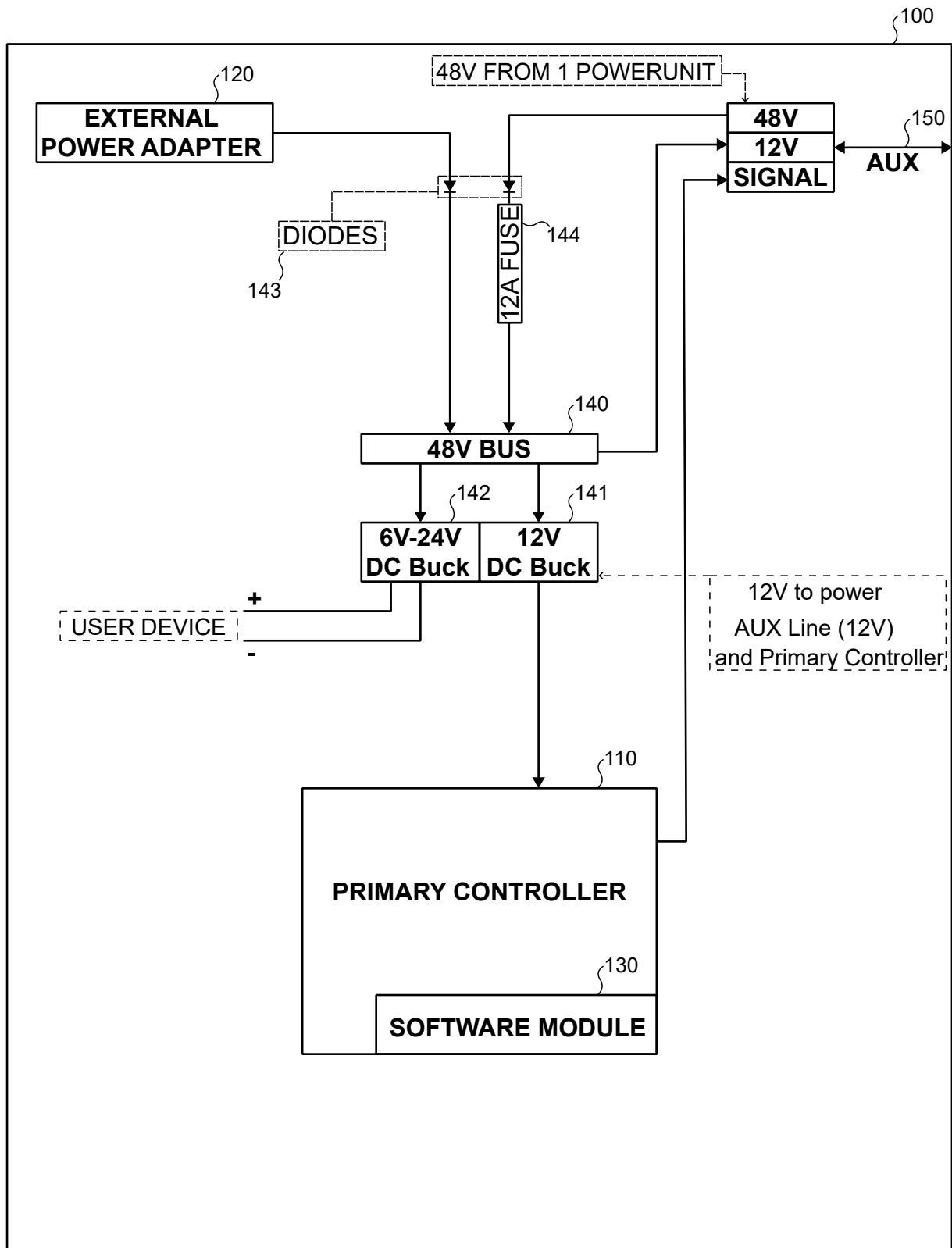
FIG 2. Central Controller Unit (100)
