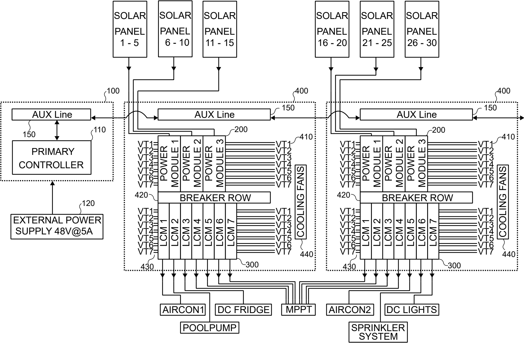
FIG 1: System-Level Block Diagram of Modular DC Power Distribution System
