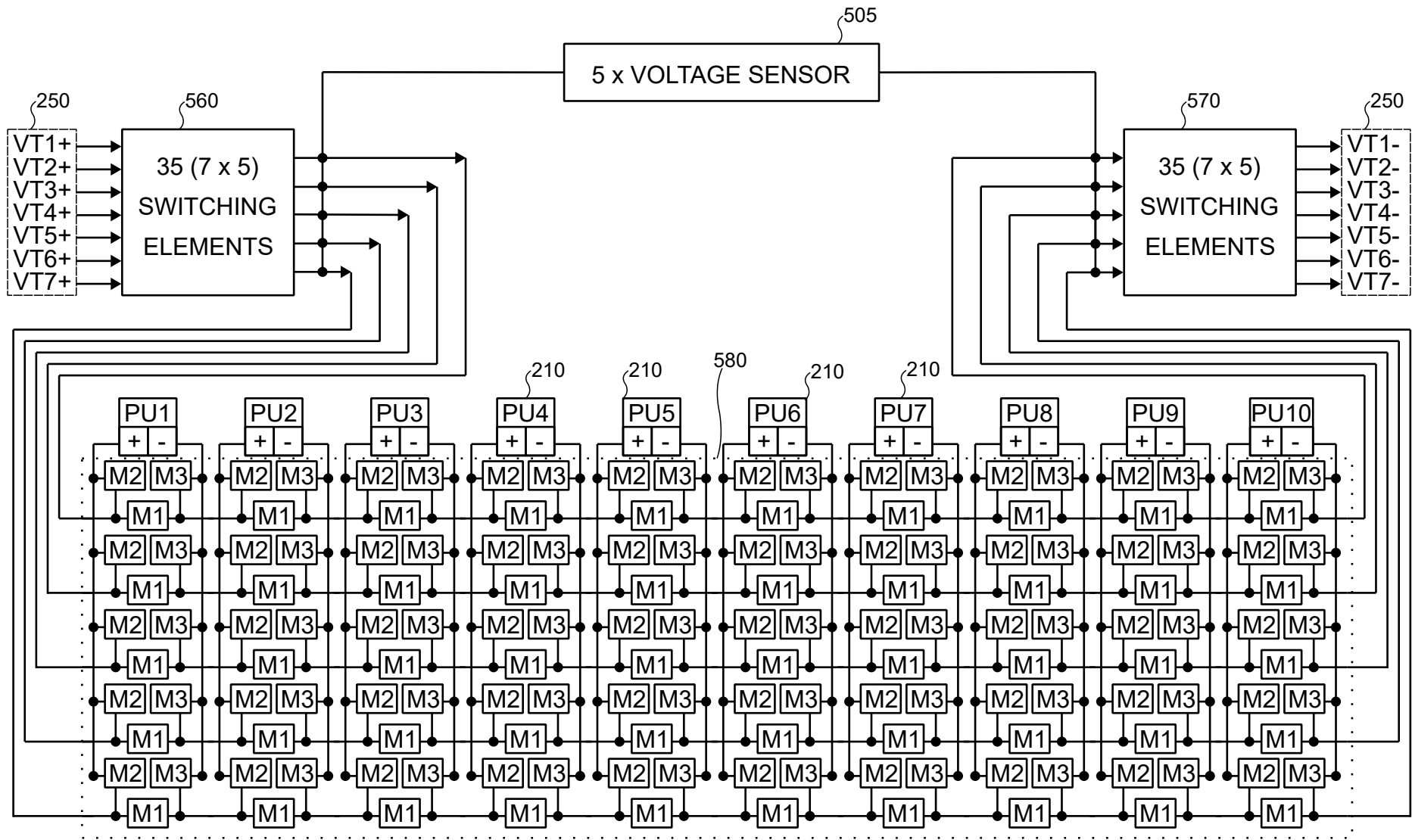
FIG. 4B: SWITCHING MATRIX SECOND EMBODIMENT (550)
