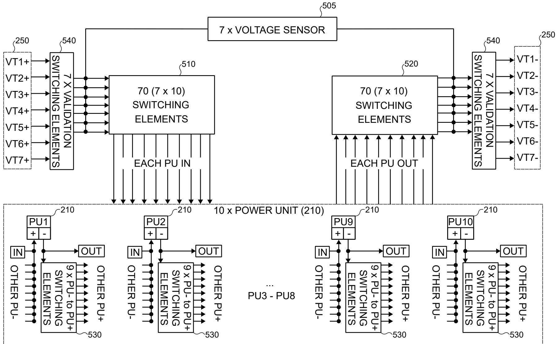
FIG. 4A: SWITCHING MATRIX FIRST EMBODIMENT (500)
