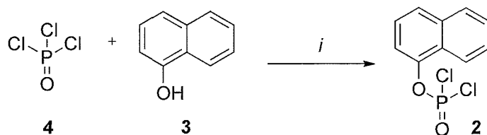
Scheme 1. Reagents and Conditions: (i) 1-naphthol (3), phosphorus oxychloride (4), dry \text{Et}_2\text{O} , dry \text{Et}_3\text{N} , -78\text{ }^\circ\text{C} ., 30min. then R.T., 3h.
