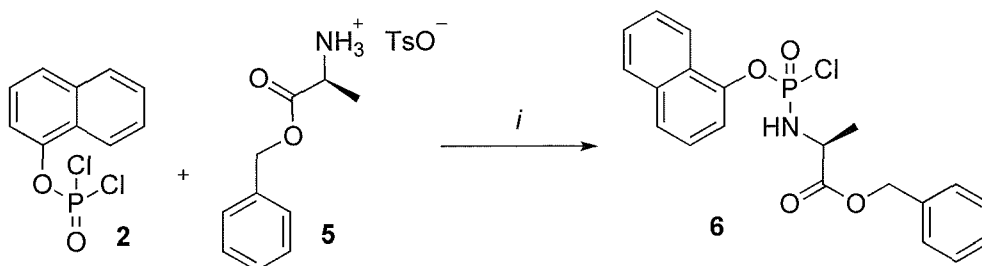
Scheme 2. Reagents and Conditions: (i) dry \text{Et}_3\text{N} , \text{CH}_2\text{Cl}_2 , -78\text{ }^\circ\text{C} ., 1h then R.T., 3h.
