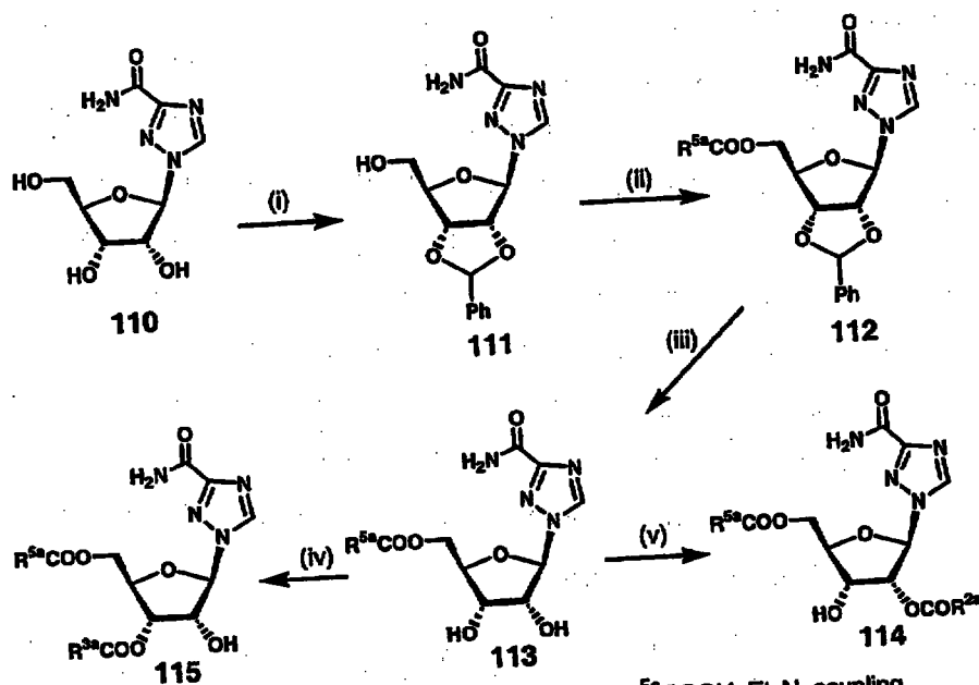
Scheme I (5'-Substitutions)
