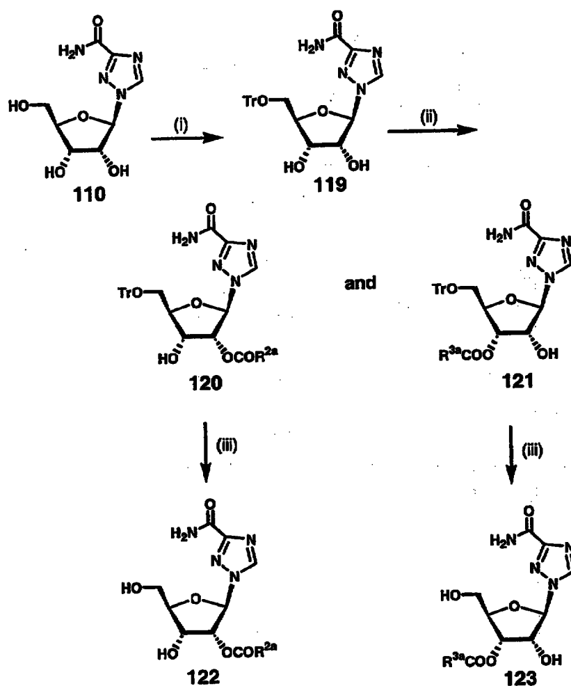
Scheme III (2' and 3'-Substitutions)
