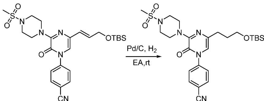
[0602] 4-(5-(3-(( tert -Butyldimethylsilyl)oxy)propyl)-3-(4-(methylsulfonyl)piperazin-1-yl)-2-oxopyrazin-1(2H)-yl)benzonitrile The procedure for preparing Intermediate 3-4 was used with the product from the previous step (900 mg, 1.0 equiv) to afford 600 mg of the title compound as a yellow oil.
