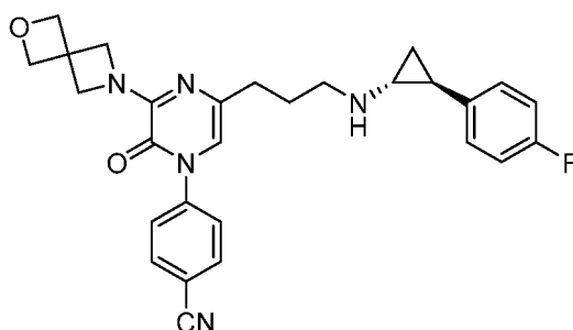
4-[5-(3-(((1 R ,2 S )-2-[4-fluorophenyl]cyclopropyl)amino)propyl)-2-oxo-3-(2-oxa-6-azaspiro[3.3]heptan-6-yl)pyrazin-1(2 H )-yl]benzonitrile
