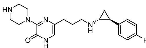
5-[3-((1 R ,2 S )-2-(4-fluorophenyl)cyclopropyl)amino)propyl]-3-[piperazin-1-yl]pyrazin-2(1 H )-one
