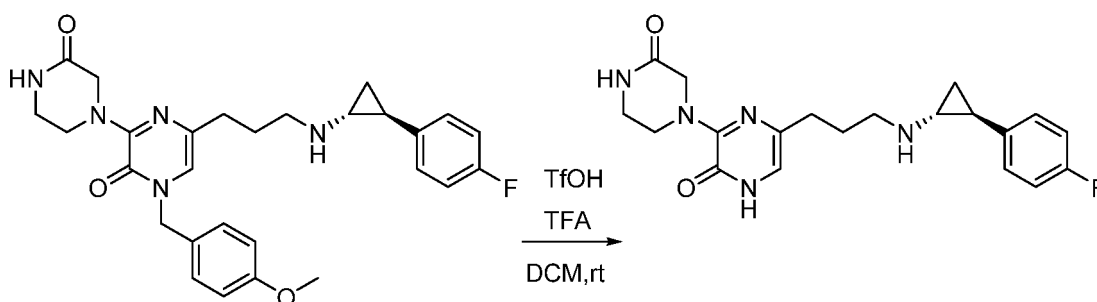
5-[3-(((1 R ,2 S )-2-(4-fluorophenyl)cyclopropyl)amino)propyl]-3-[3-oxopiperazin-1-yl]pyrazin-2(1 H )-one
