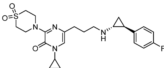
1-Cyclopropyl-3-[1,1-dioxidothiomorpholino]-5-[3-([(1 R ,2 S )-2-(4-fluorophenyl)cyclopropyl]amino)propyl]pyrazin-2(1 H )-one
