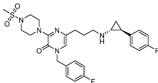
1-(4-fluorobenzyl)-5-[3-([(1 R ,2 S )-2-(4-fluorophenyl)cyclopropyl]amino)propyl]-3-[4-(methylsulfonyl)piperazin-1-yl]pyrazin-2(1 H )-one
