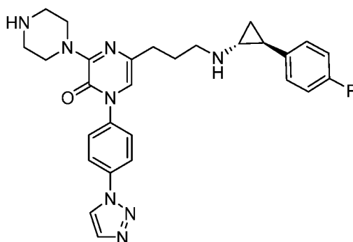
1-[4-(1 H -1,2,3-triazol-1-yl)phenyl]-5-[3-([(1 R ,2 S )-2-(4-fluorophenyl)-cyclopropyl]amino)propyl]-3-[piperazin-1-yl]pyrazin-2(1 H )-one
