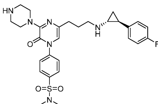
4-[5-(3-((1 R ,2 S )-2-[4-fluorophenyl]cyclopropyl)amino)propyl)-2-oxo-3-(piperazin-1-yl)pyrazin-1(2 H )-yl]- N,N -dimethylbenzenesulfonamide
