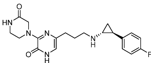
5-[3-(((1 R ,2 S )-2-(4-fluorophenyl)cyclopropyl)amino)propyl]-3-[3-oxopiperazin-1-yl]pyrazin-2(1 H )-one
