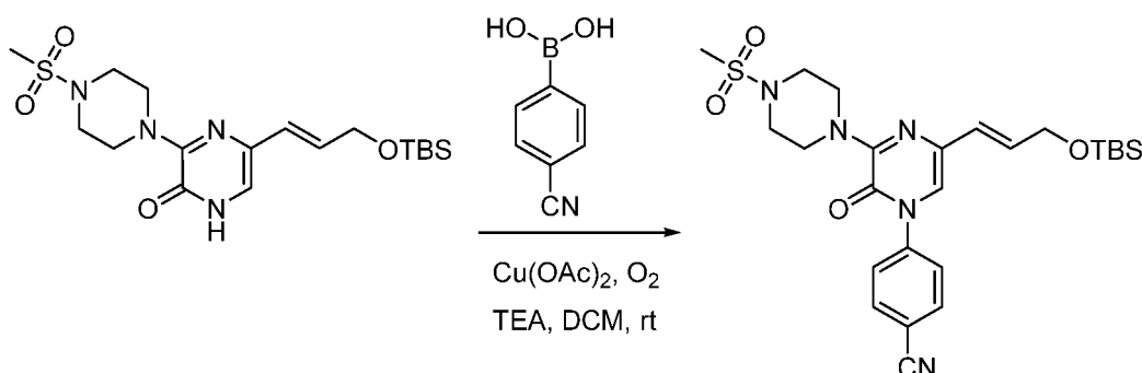
[0601] (E)-4-(5-(3-(( tert -butyldimethylsilyl)oxy)prop-1-en-1-yl)-3-(4-(methylsulfonyl)piperazin-1-yl)-2-oxopyrazin-1(2H)-yl)benzonitrile
