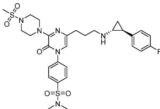
4-[5-(3-[(1 R ,2 S )-2-(4-Fluorophenyl)cyclopropyl]amino)propyl]-3-(4-methanesulfonylpiperazin-1-yl)-2(1 H )-oxopyrazin-1-yl]- N,N -dimethylbenzene-1-sulfonamide
