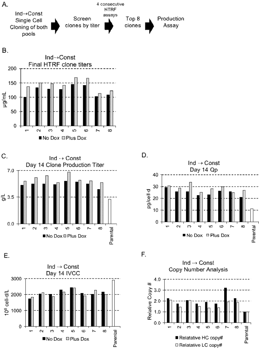
Figure 5. Single cell cloning of Ind→Const supertransfected pools
