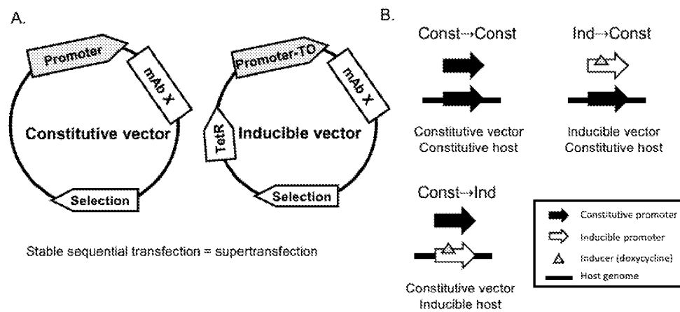
Figure 1. An overview of the supertransfection expression constructs and the three different supertransfection approaches.
