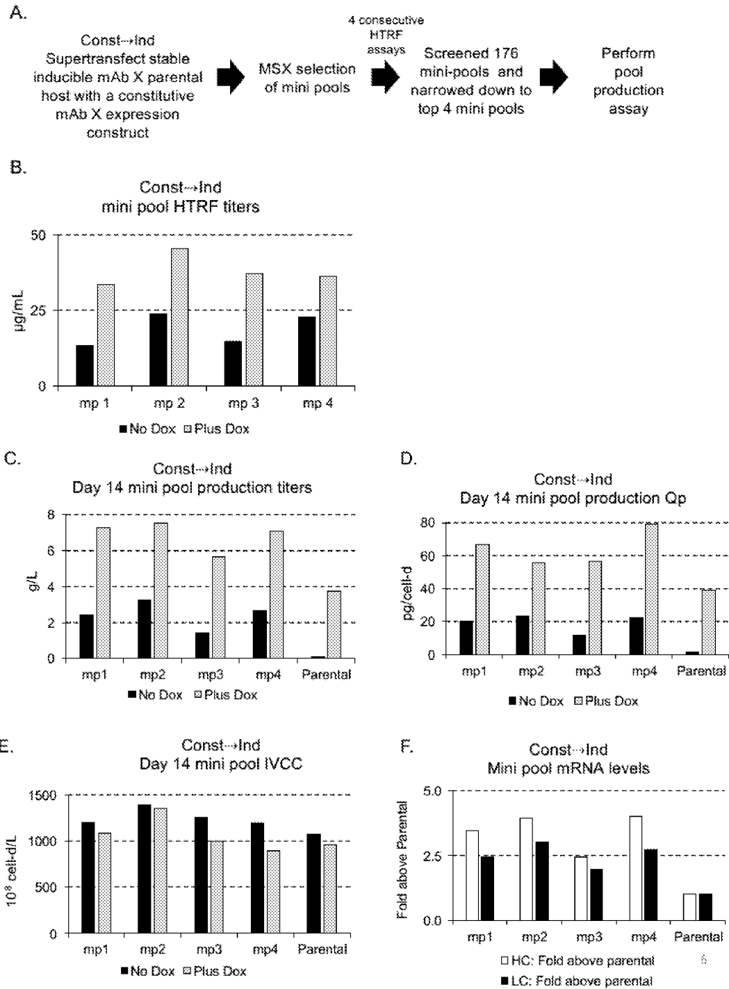
Figure 6. Const→Ind supertransfection overview
