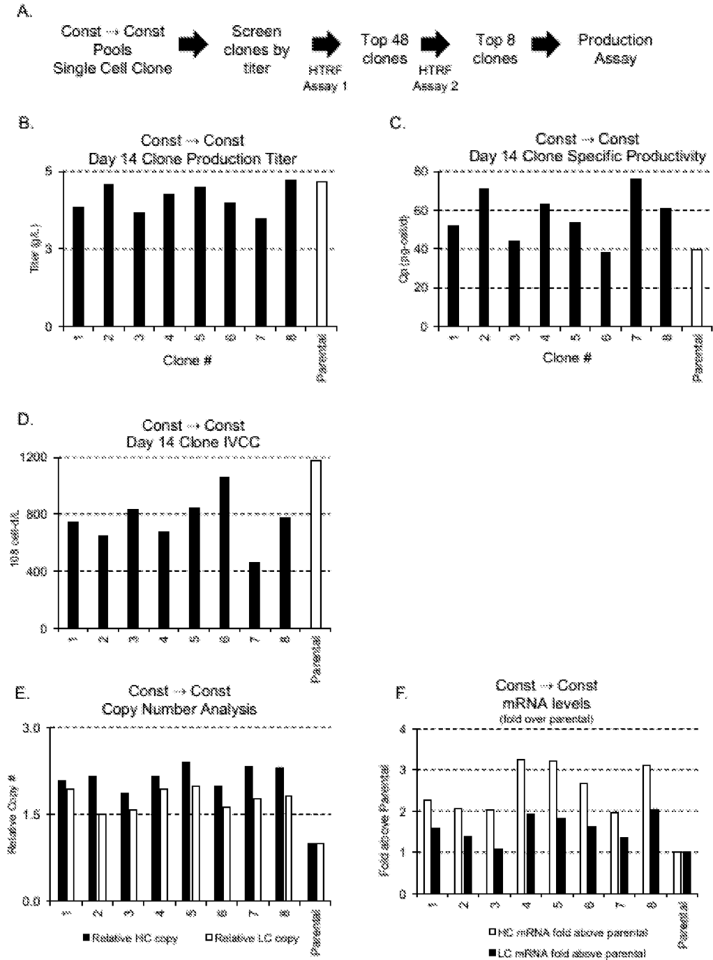
Figure 3. Single cell cloning of Const→Const pools to obtain high titer supertransfected clones.
