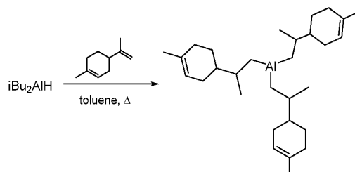
Scheme 8.
