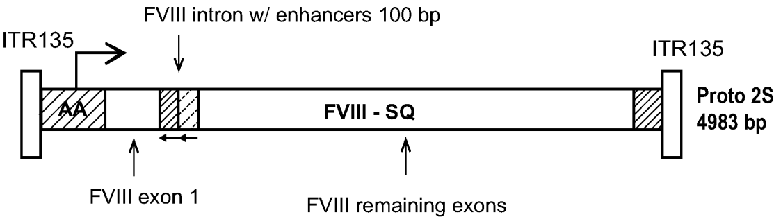
Schematic of Proto 2S
