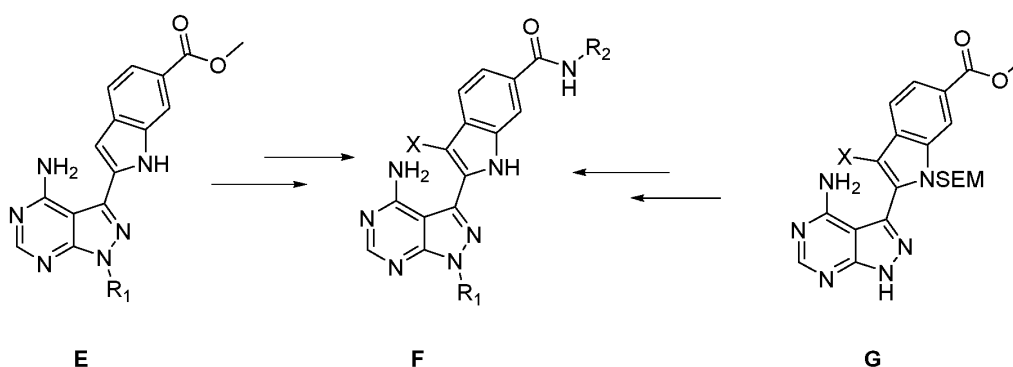
Scheme 2 – Elaboration of Indolyl Pyrazolopyrimidines
