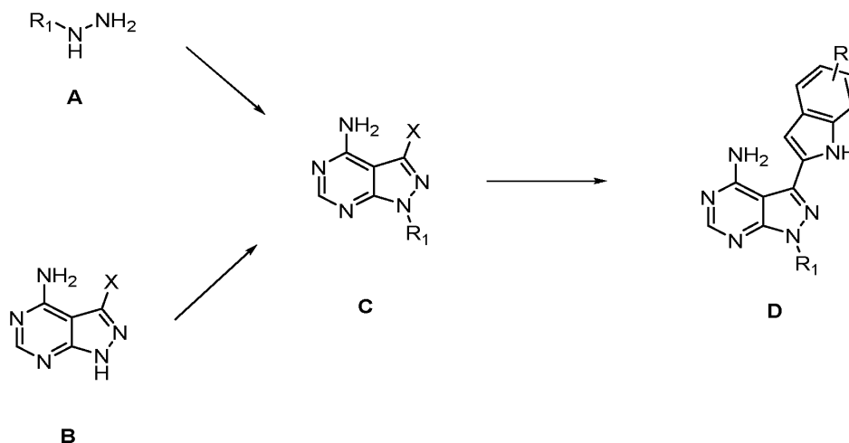
Scheme 1 – Preparation of Indolyl Pyrazolopyrimidines D
