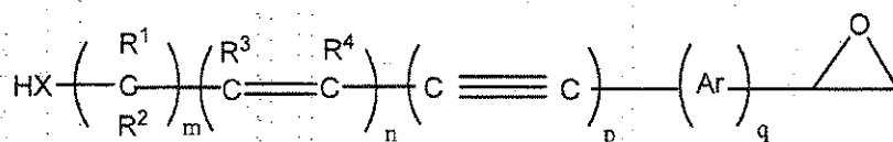
formula (Ib)
