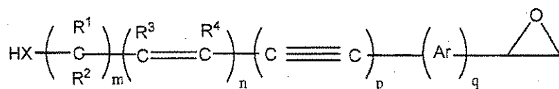
formula (Ib)
