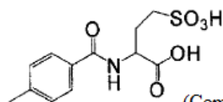
(Compound 50),
