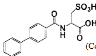
(Compound 47),
