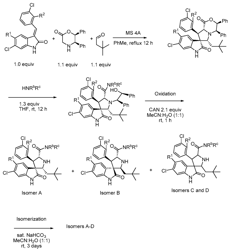
Scheme 10
