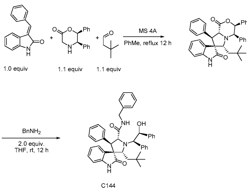
Scheme 16
