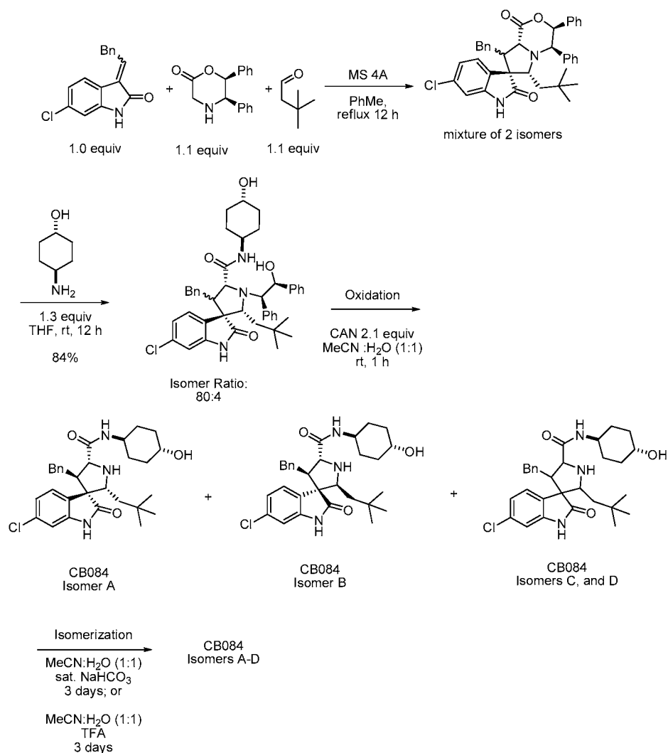
Scheme 15
