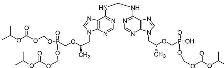
Mixed Dimer
