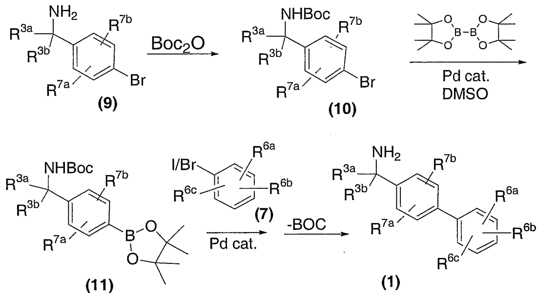
SCHEME 2b
