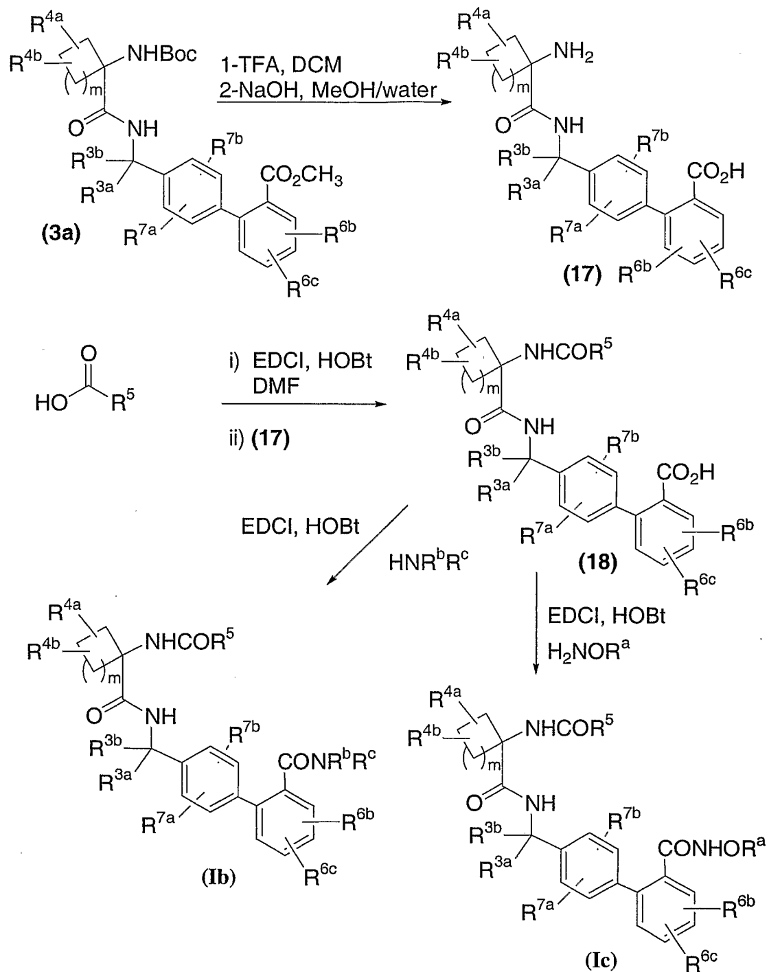
SCHEME 3
