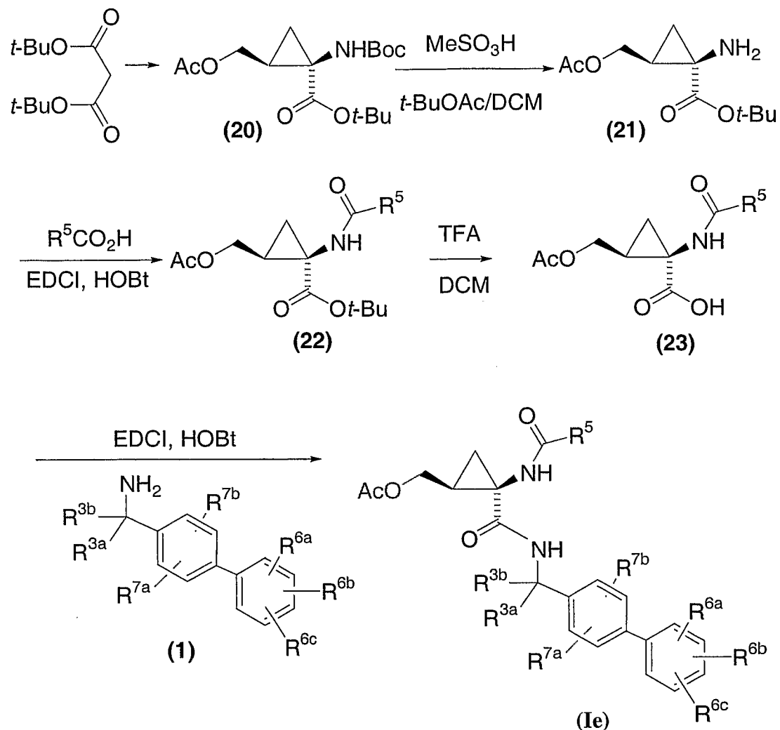
SCHEME 5
