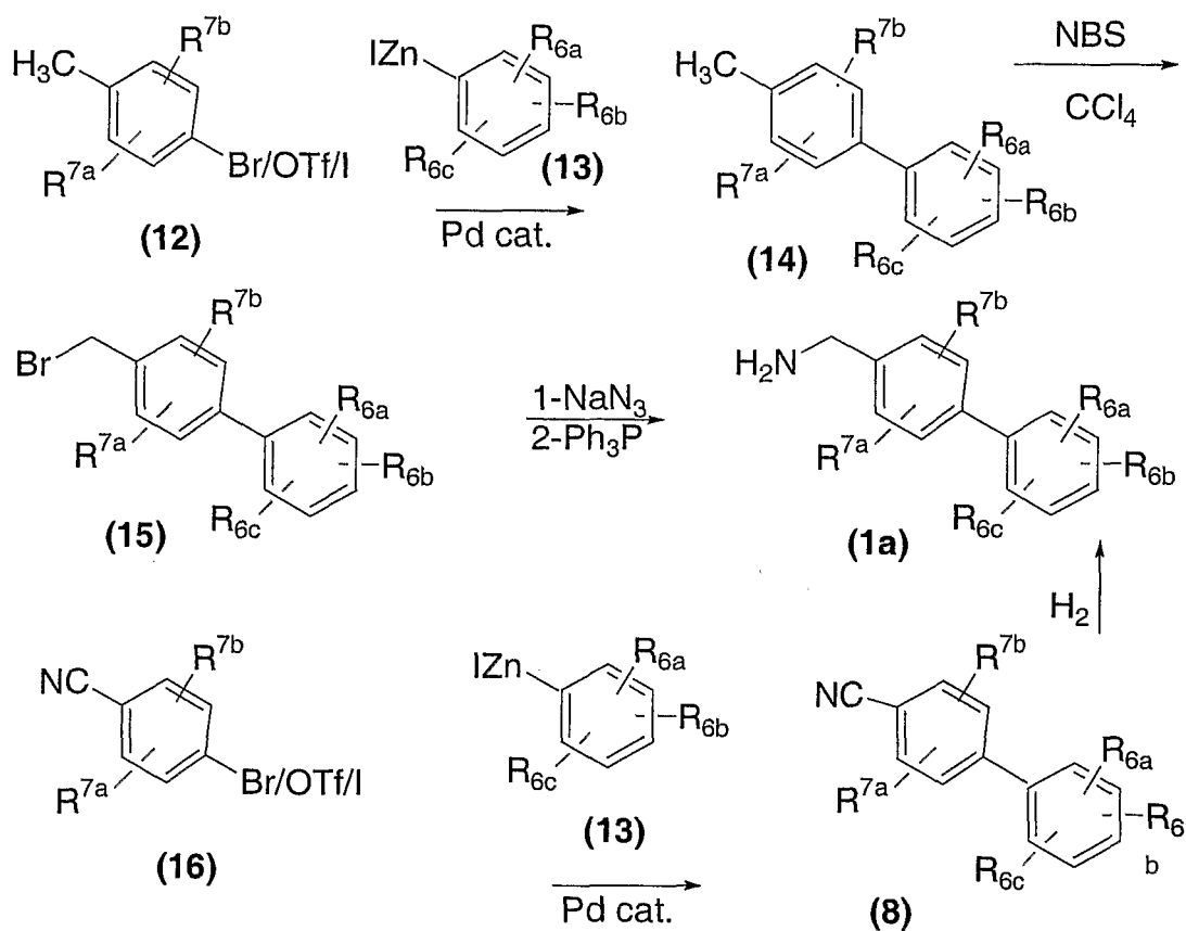
SCHEME 2c
