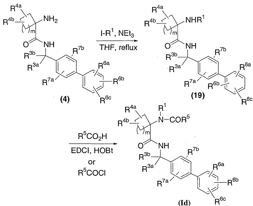
SCHEME 4
