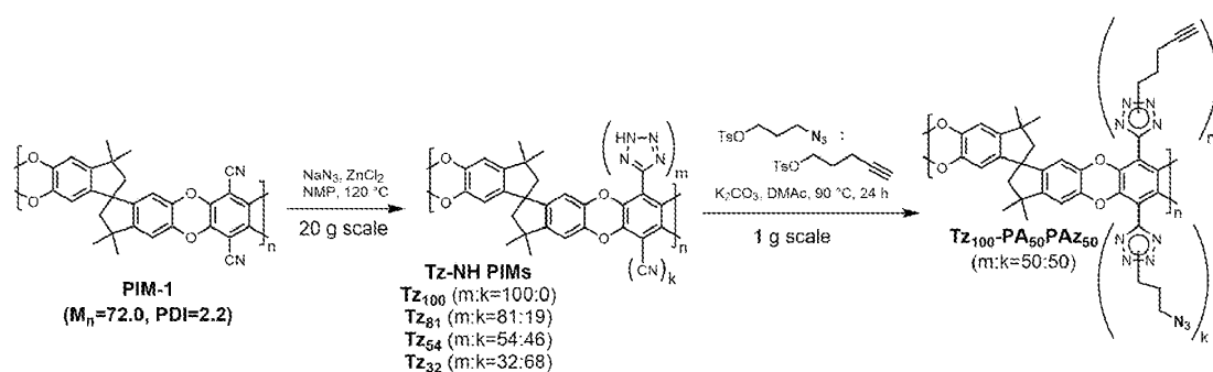
[000419] Reaction Scheme 12.
