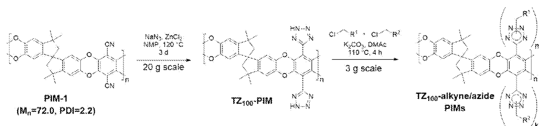
[000421] Reaction Scheme 13.
