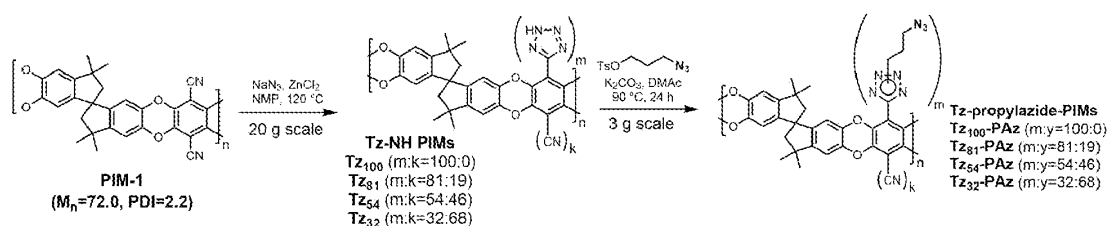
[000419] Reaction Scheme 12.
