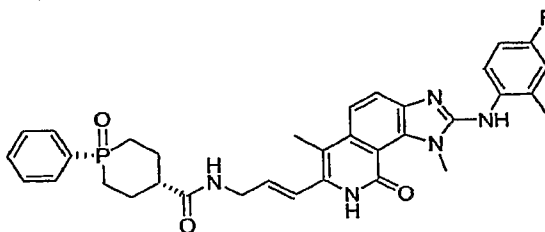
Compound 17
