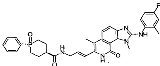
Compound 16
