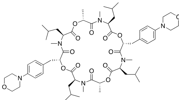
(Emodepside)
