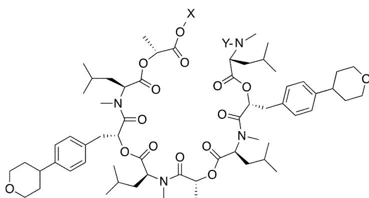
(II-5b)
