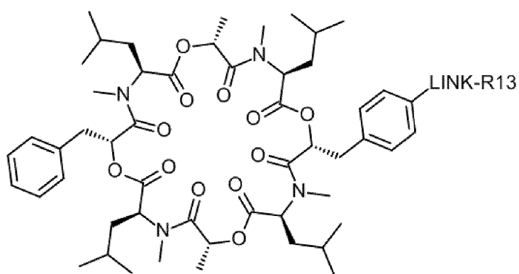
(I-7)
