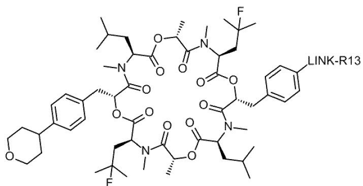
(I-7)
