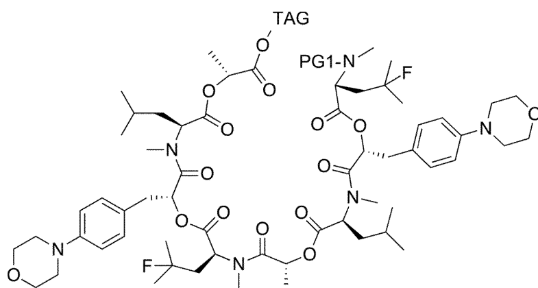
(II-3)
