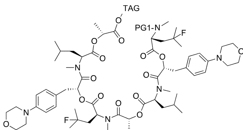
(II-3)
