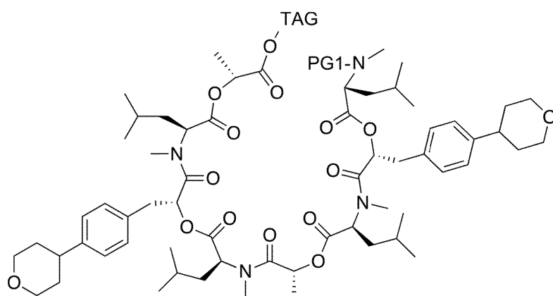
(II-5)
