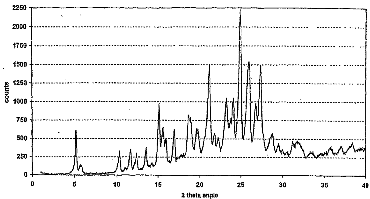
Powder X-ray Diffraction Pattern of 1,4-Dioxane Hemisolvate
