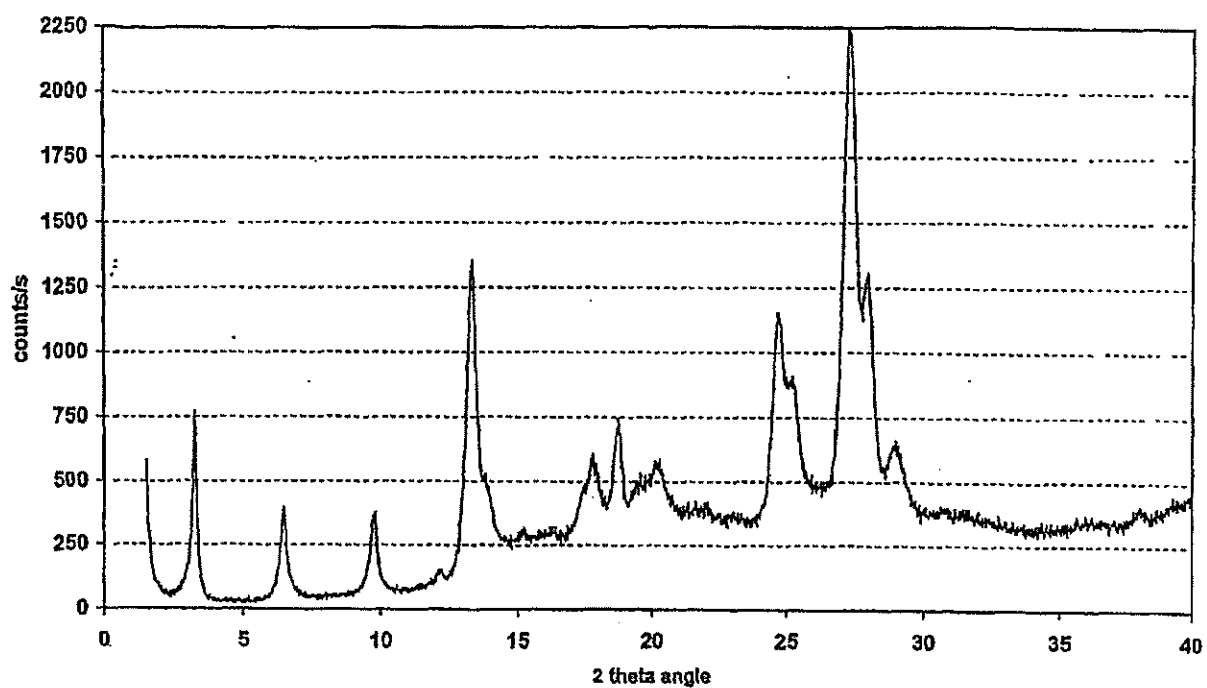
Powder X-ray Diffraction Pattern of Form C
