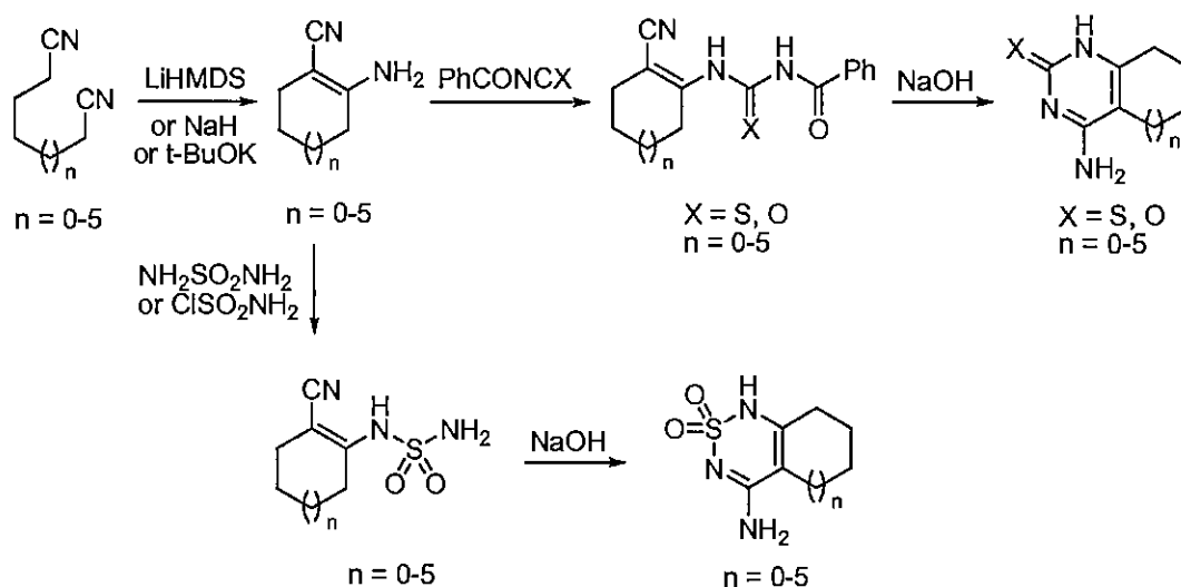
Scheme 9
