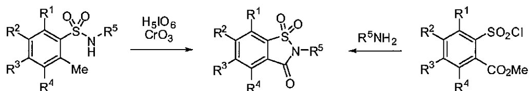
Scheme 12
