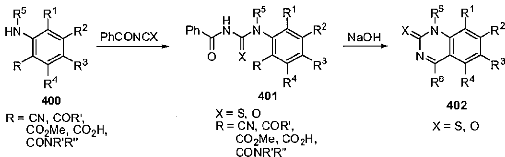
Scheme 6
