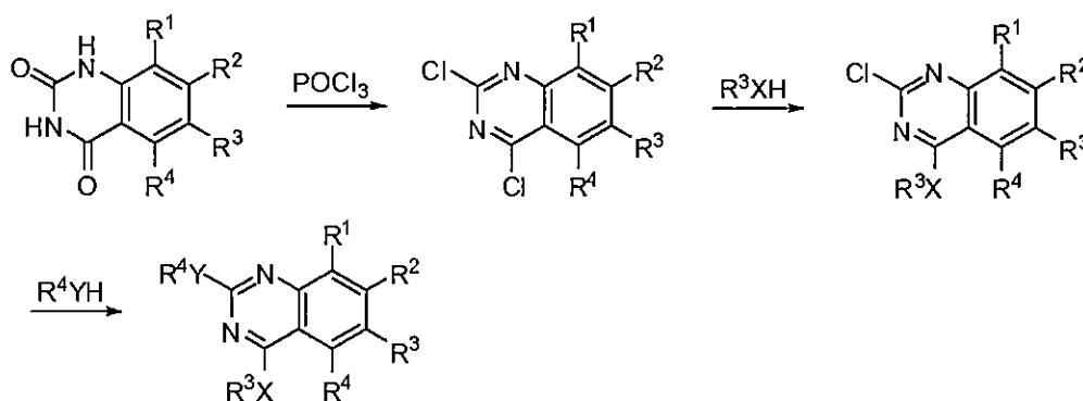
Scheme 8
