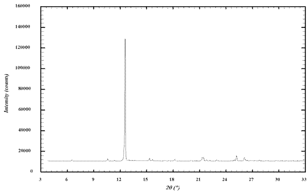
FIG 33. XRPD pattern of 1-hydroxy-2-naphtic acid salt (form 1)
