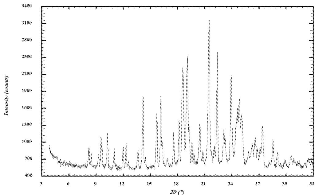
FIG 1. XRPD pattern of naphthalene-1,5-disulfonic acid salt (form 1)
