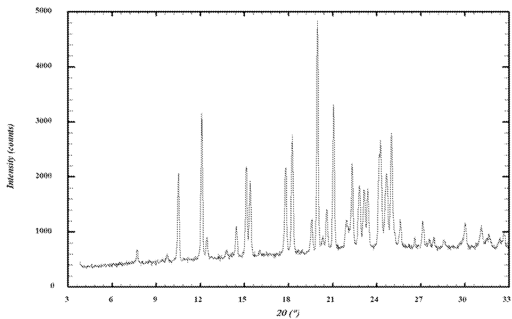
FIG 27. XRPD pattern of adipic acid salt (form 1)
