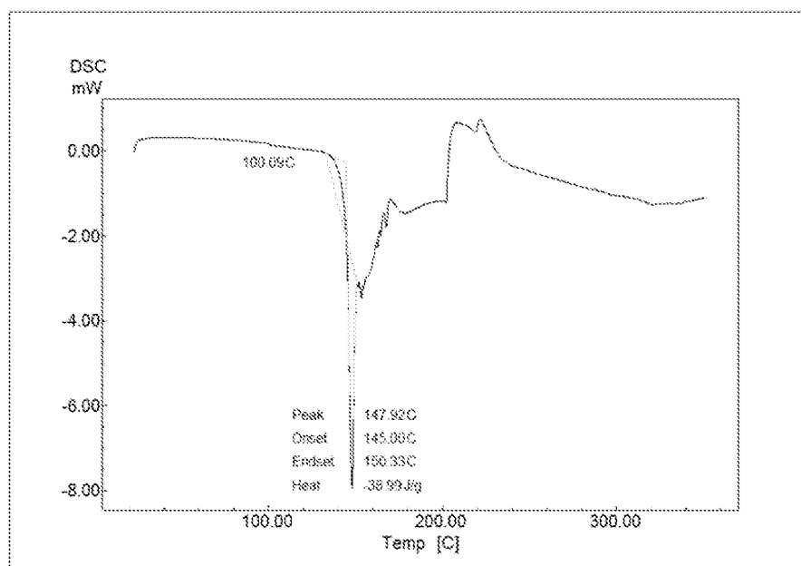
FIG 14. DSC thermogram of malonic acid salt (form 1)
