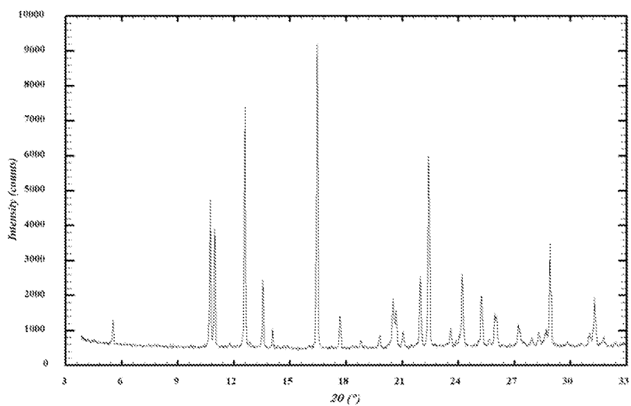
FIG 35. XRPD pattern of hydrochloric acid salt (form 1)
