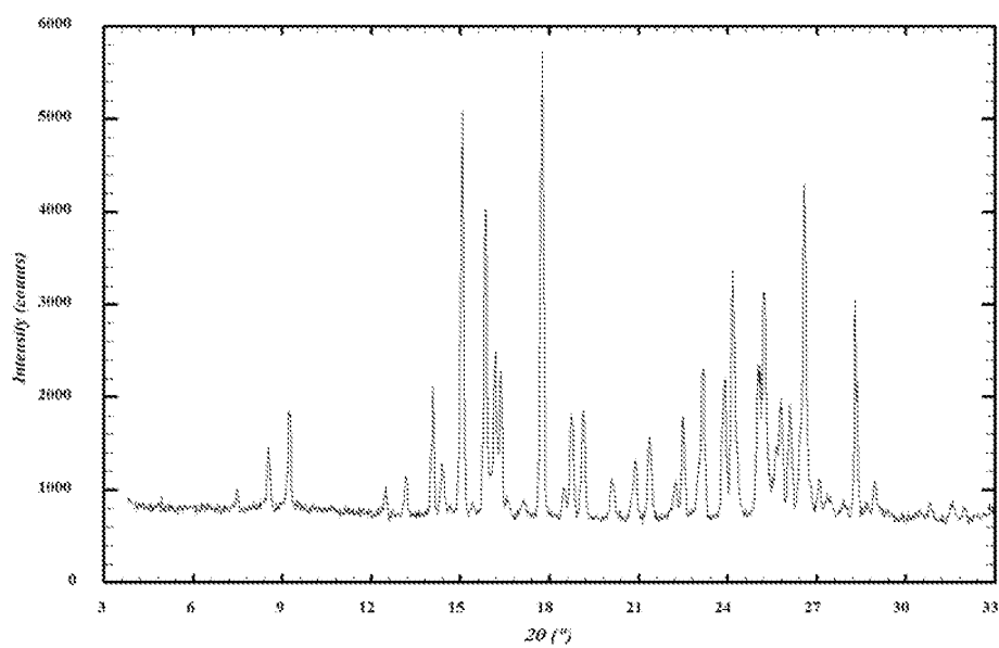
FIG 9. XRPD pattern of saccharin acid salt (form 2)
