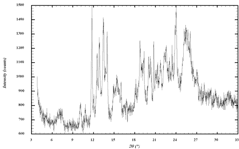
FIG 15. XRPD pattern of L-tartaric acid salt (form 1)
