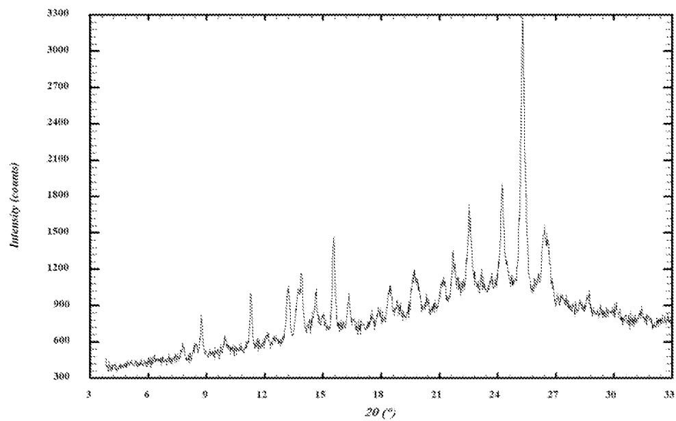
FIG 19. XRPD pattern of fumaric acid salt (form 1)
