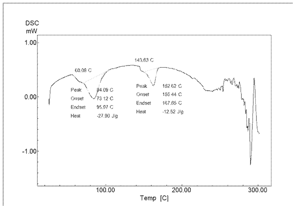
FIG 2. DSC thermogram of naphthalene-1,5-disulfonic acid salt (form 1)
