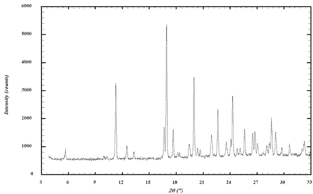
FIG 29. XRPD pattern of hydrobromic acid salt (form 1)
