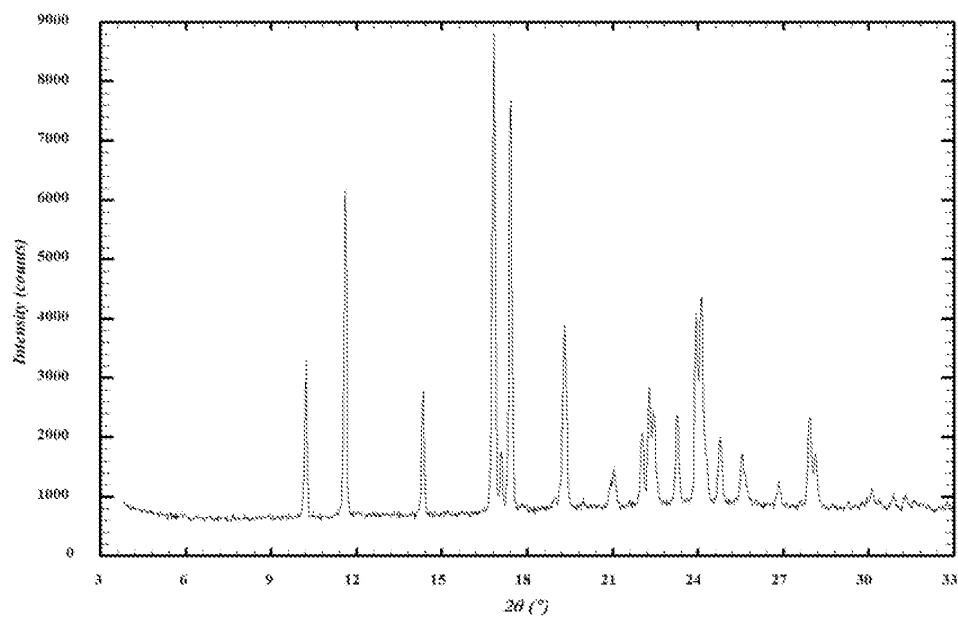
FIG 11. XRPD pattern of maleic acid salt (form 1)
