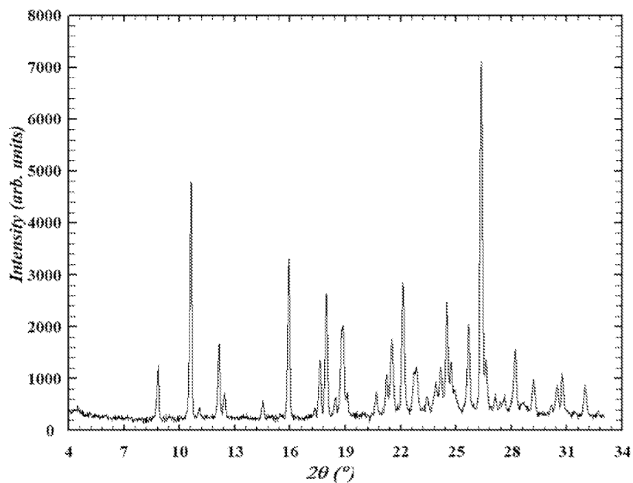
FIG 21. XRPD pattern of fumaric acid salt (form 2)
