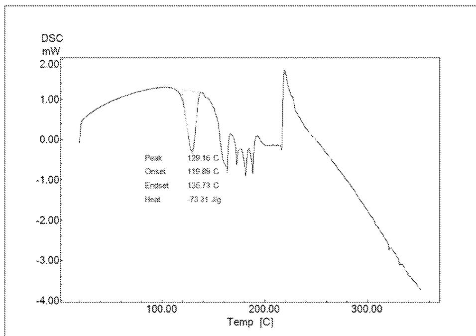
FIG 34. DSC thermogram of 1-hydroxy-2-naphtic acid salt (form 1)
