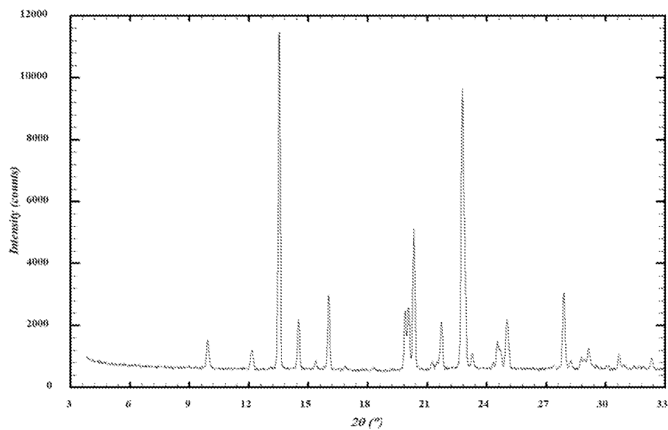
FIG 3. XRPD pattern of ethane-1,2-disulfonic acid salt (form 1)
