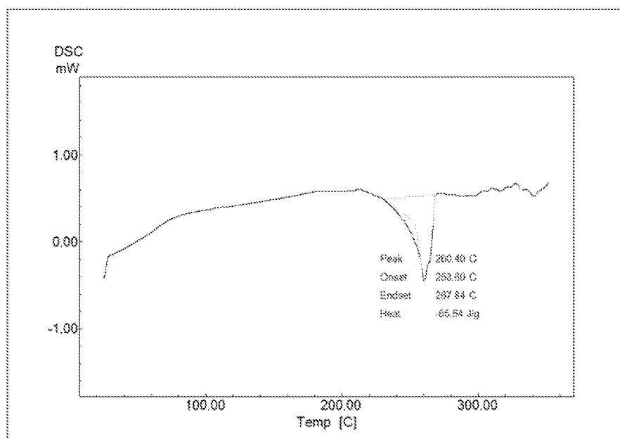
FIG 4. DSC thermogram of ethane-1,2-disulfonic acid salt (form 1)
