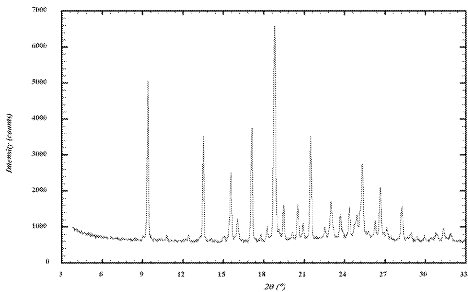
FIG 7. XRPD pattern of saccharin acid salt (form 1)
