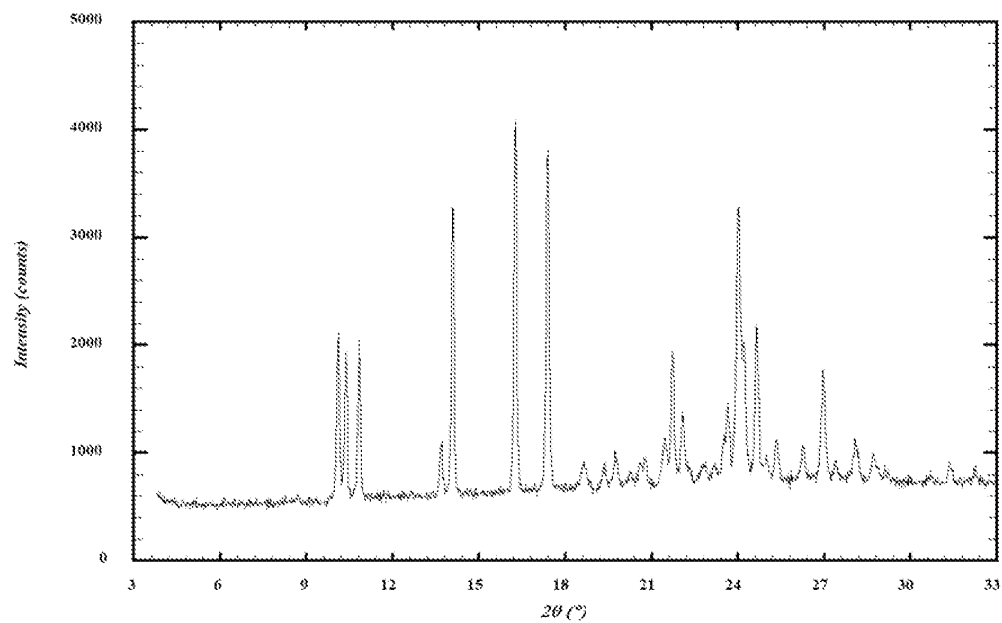
FIG 13. XRPD pattern of malonic acid salt (form 1)
