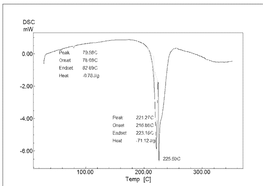
FIG 6. DSC thermogram of oxalic acid salt (form 1)
