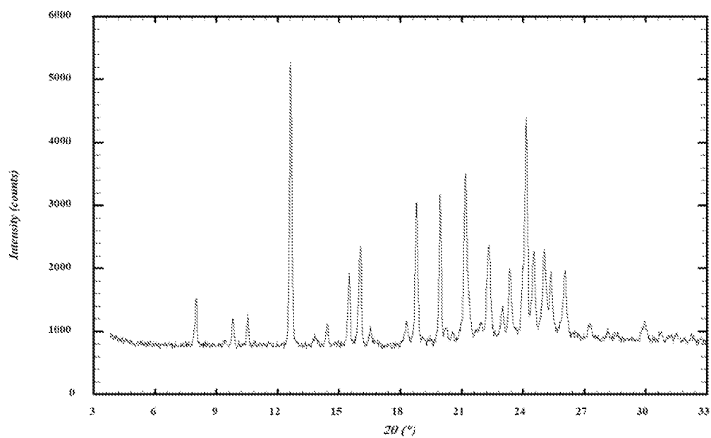
FIG 25. XRPD pattern of glutaric acid salt (form 1)
