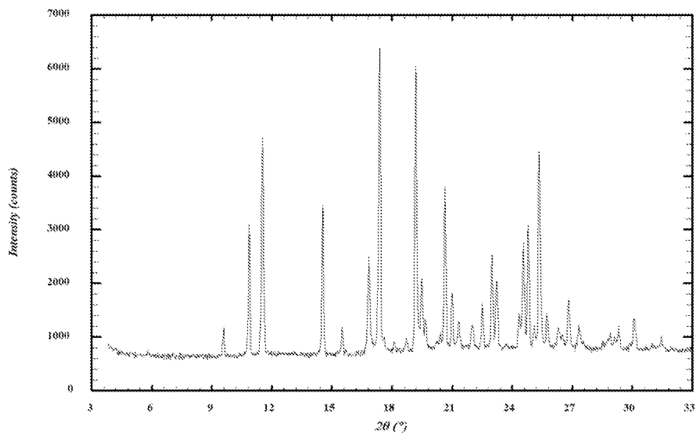
FIG 23. XRPD pattern of glycolic acid salt (form 1)
