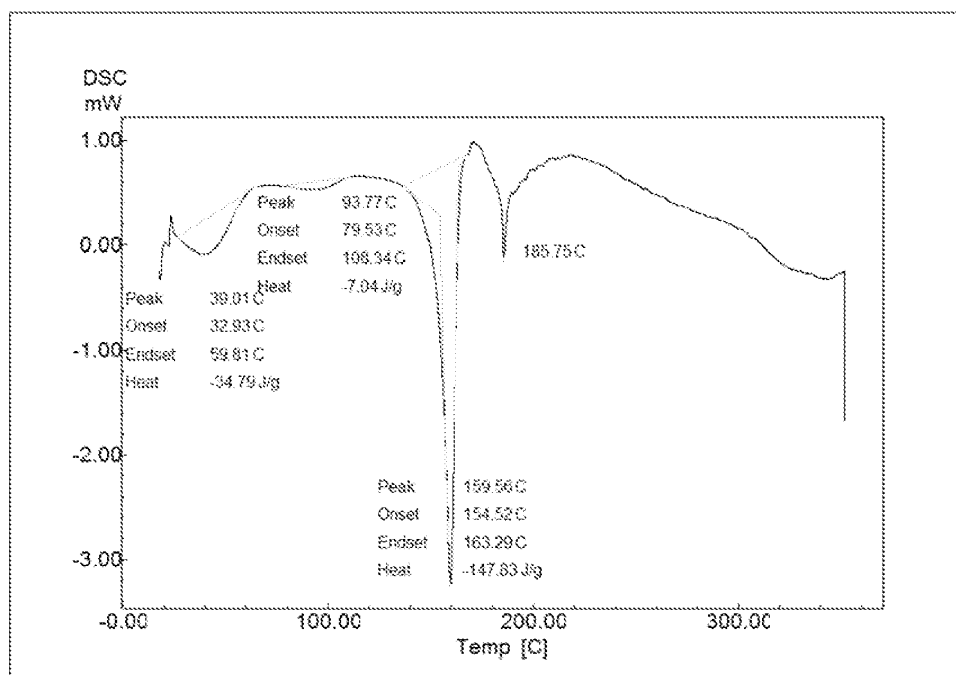
FIG 32. DSC thermogram of mucic acid salt (form 1)
