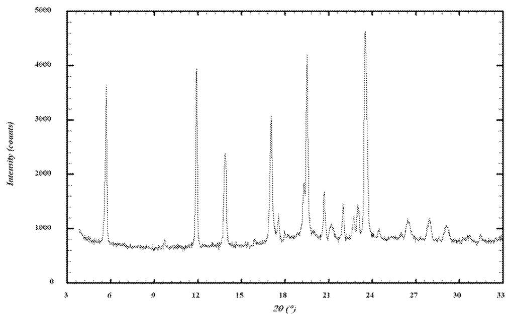
FIG 31. XRPD pattern of mucic acid salt (form 1)
