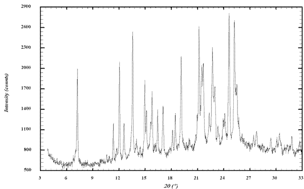
FIG 17. XRPD pattern of L-tartaric acid salt (form 2)
