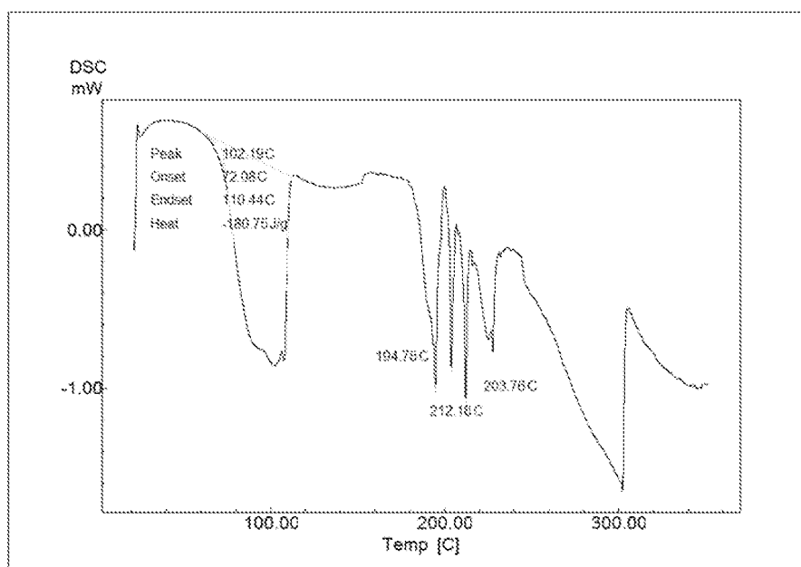
FIG 22. DSC thermogram of fumaric acid salt (form 2)
