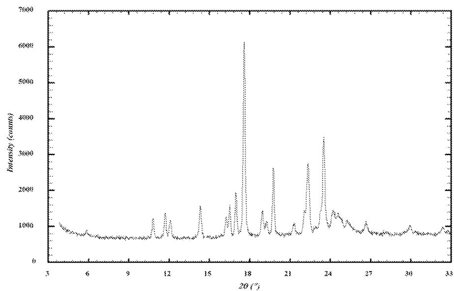
FIG 5. XRPD pattern of oxalic acid salt (form 1)
