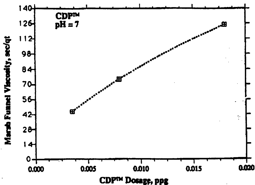
Marsh Funnel Viscosity vs. CDP™ Dosage.
