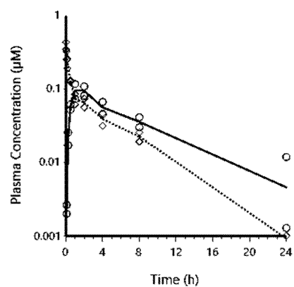
FIGS. 15 - 19: PK curves following IV (0.5 mg/kg) [dotted line] and PO (1 mg/kg) [solid line] dosing.
