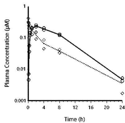
FIGS. 8 - 14: PK curves following IV (0.5 mg/kg) [dotted line] and PO (1 mg/kg) [solid line] dosing.
