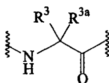
Formula IIa
