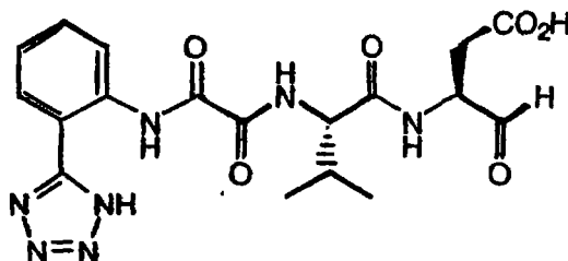
(3S)-3-[N-(N'-(2-(1H-Tetrazol-5-yl)Phenyl)Oxamyl)Valinyl] Amino-4-Oxobutanoic Acid
