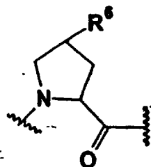
IIId
