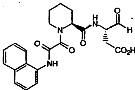
(3S)-3-[N-(N'-(1-Naphthyl)Oxamyl)Homoprolinyl] Amino-4-Oxobutanoic Acid
