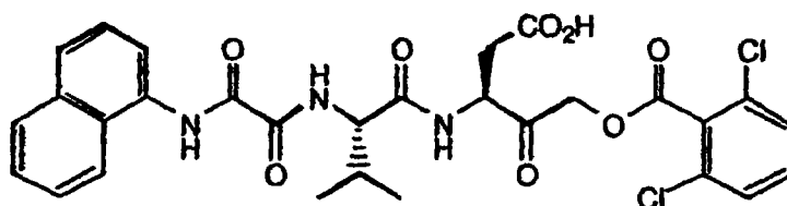
10 (3S)-3-[N-(N'-(1-Naphthyl)Oxamyl)Valinyl] Amino-5-(2',6'-Dichlorobenzoyloxy)-4-Oxopentanoic Acid
