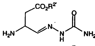
Formula Vb;
