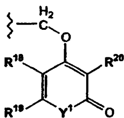
IIIa
