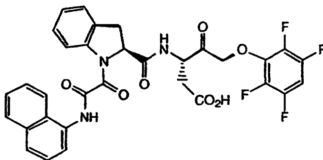
(3S)-3-[N-(N'-(1-Naphthyl)Oxamyl)]Indoline-2-Carbonyl] Amino-5-(2',3',5',6'-Tetrafluorophenoxy)-4-Oxopentanoic Acid
