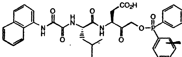
(3S)-3-[N-(N'-(1-Naphthyl)Oxamyl)Leucinyl] Amino-5-(Diphenylphosphinyloxy)-4-Oxopentanoic Acid
