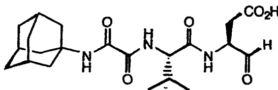
(3S)-3-[N-(N'-(1-Adamantany)Oxamyl)Valinyl]
