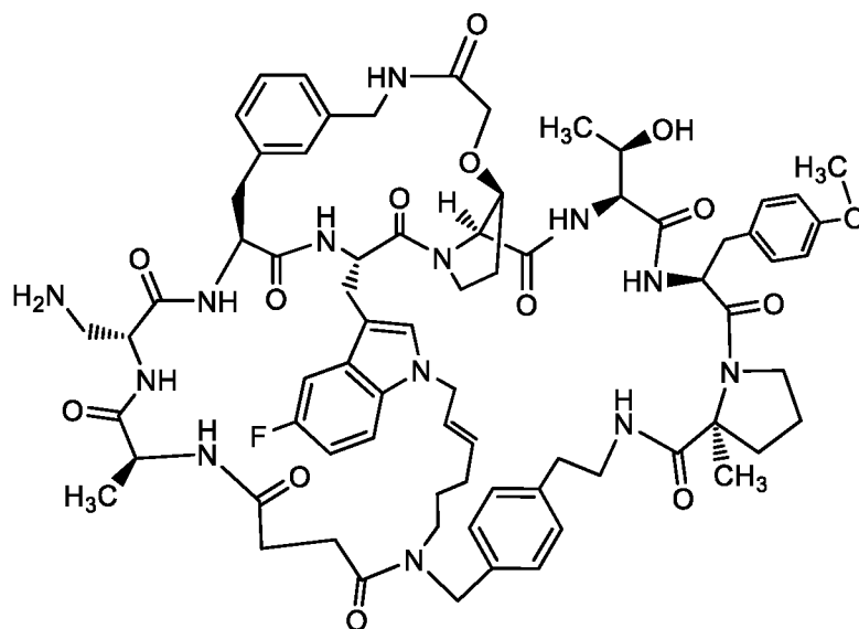
Ex-51 , (free base illustrated)
