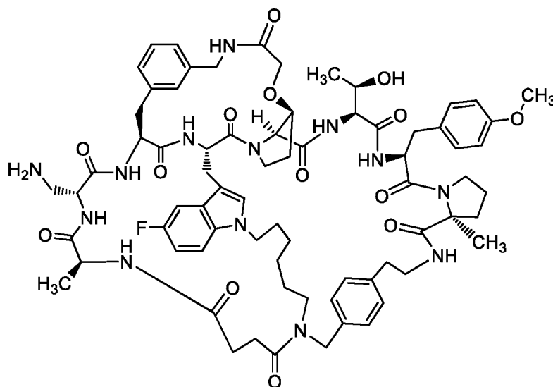
Ex-01 , (free base illustrated)
