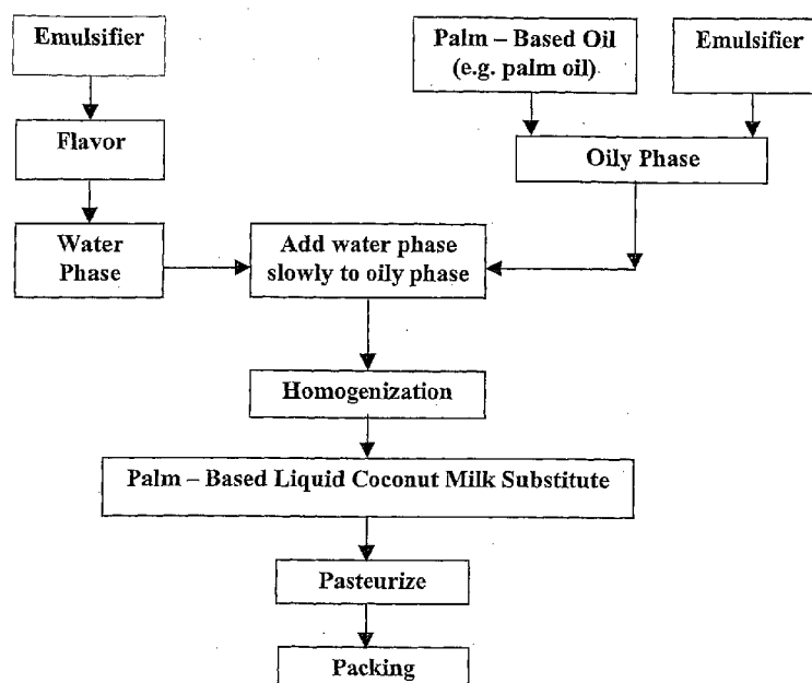
Figure 1: Flow chart illustrating the method of preparing palm-based liquid coconut milk substitute ("santan sawit") of the present invention.
