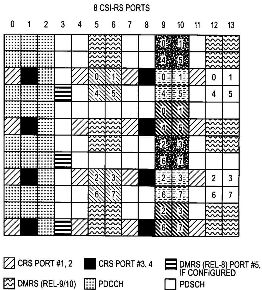
FIG. 8C (PRIOR ART)
