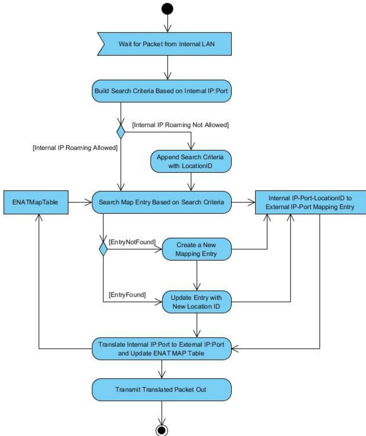
Fig 3 Ingress to LAN Packet Processing Flow
