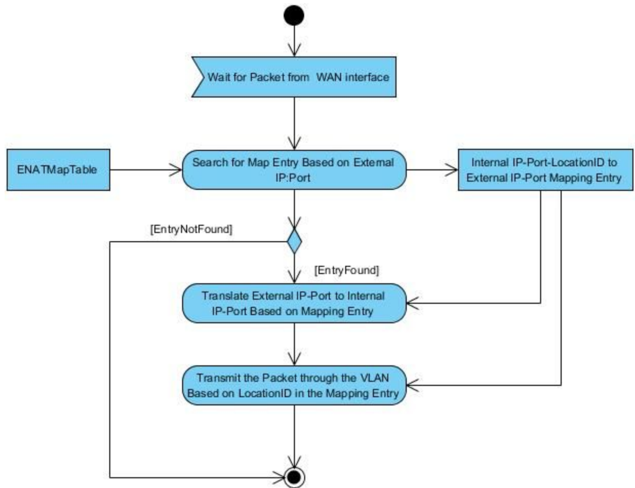
Fig 4 Ingress to WAN Packet Process Flow
