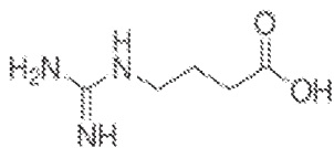
4-Guanidinobutyric acid
