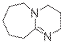
DBU = 1,8-diazabicyclo[5.4.0]undec-7-ene;
