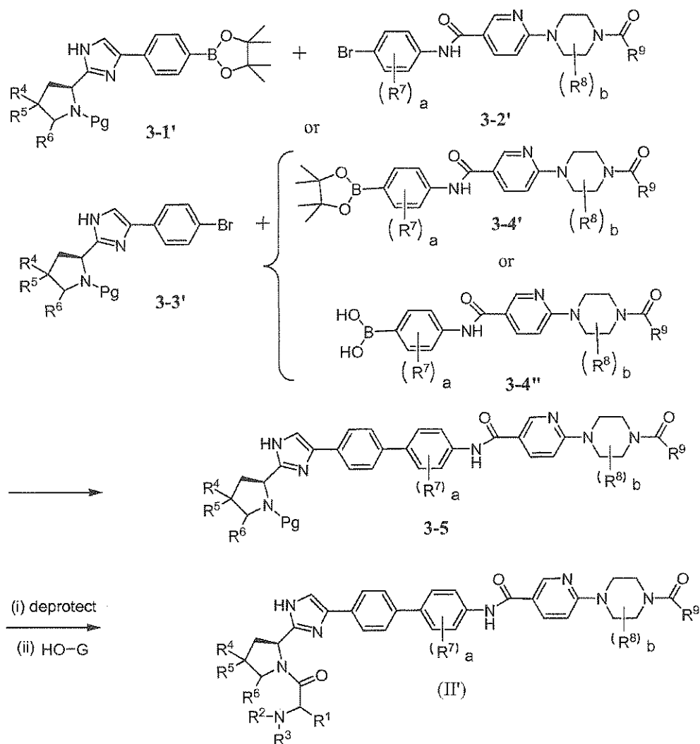
Scheme 3B
