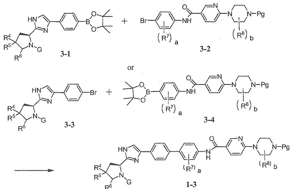
Scheme 3A
