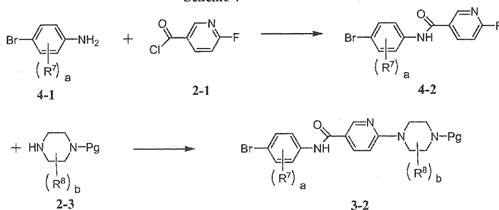
Scheme 4
