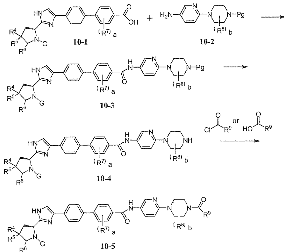
Scheme 10
