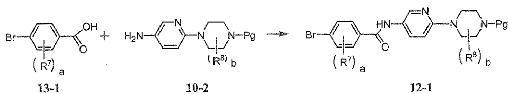
Scheme 13
