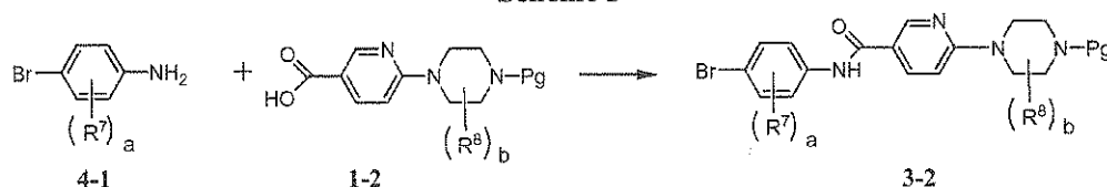
Scheme 5
