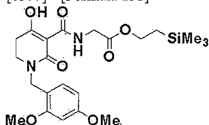
[0577] [Formula 231]
