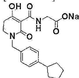
[Formula 225]
