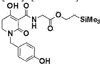
[0581] [Formula 235]
