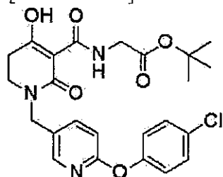
[Formula 204]
