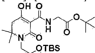
[0610] [Formula 257]
