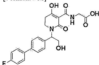
[Formula 262]
