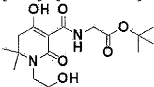
[0611] [Formula 258]
