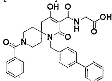
[Formula 240]
