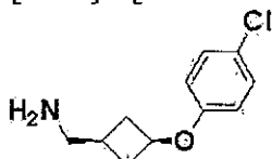
[0363] [Formula 172]
