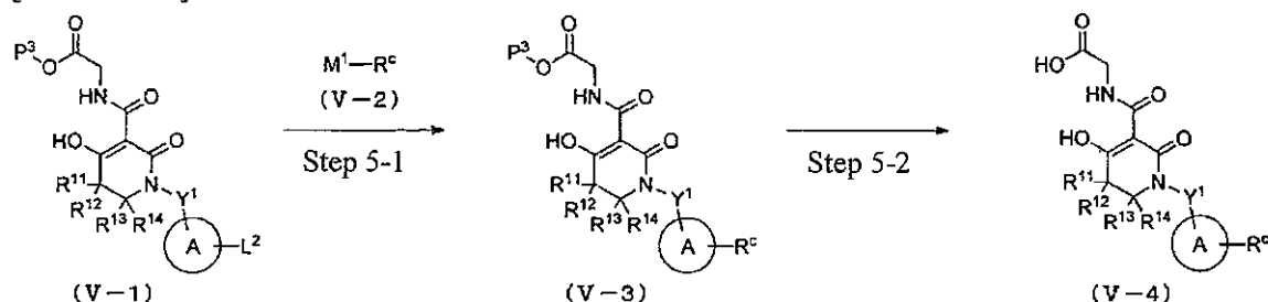
[Formula 13]
