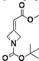
[0175] [Formula 24]
