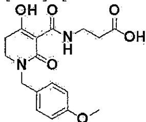
[0602] [Formula 251]
