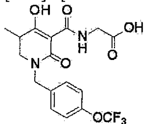
[0468] [Formula 202]
