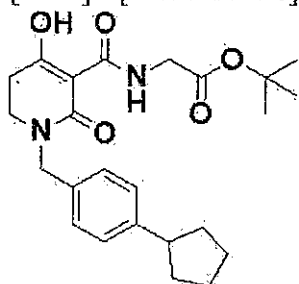
[0572] [Formula 226]
