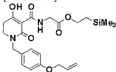
[Formula 234]
