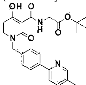
[Formula 222]
