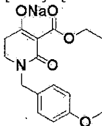
[0603] [Formula 252]
