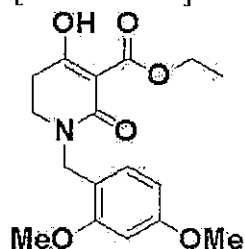
[Formula 230]
