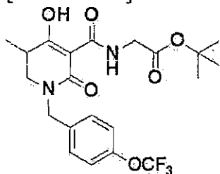
[Formula 201]
