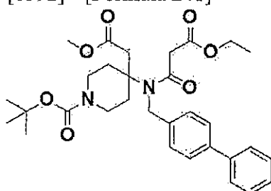
[0592] [Formula 241]
