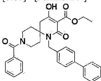
[0595] [Formula 244]
