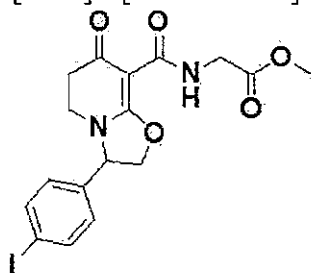
[0620] [Formula 265]
