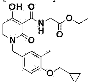
[Formula 211]
