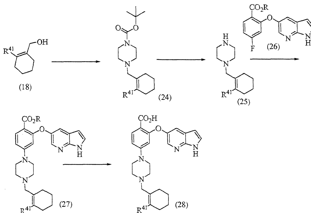
SCHEME 6
