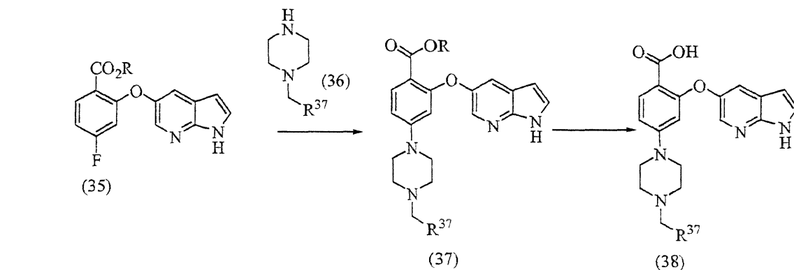
SCHEME 9
