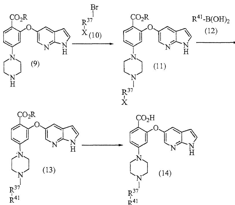
SCHEME 3
