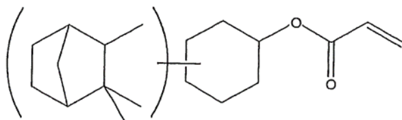
[Chemical Formula 3]
