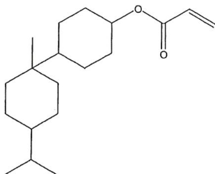
[Chemical Formula 2]
