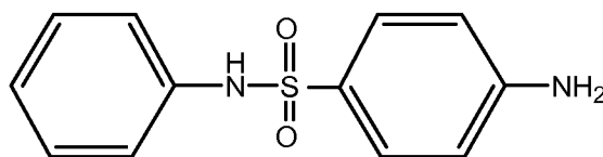
Formula (13)
