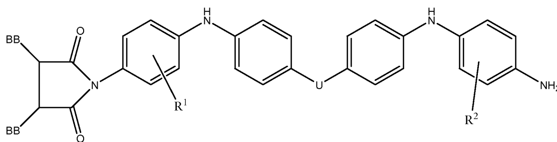
Formula (6)
