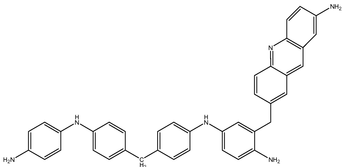
Formula (3a)
