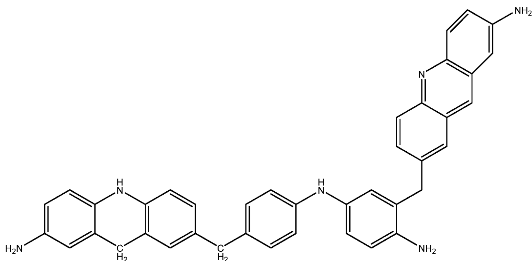
Formula (3b)
