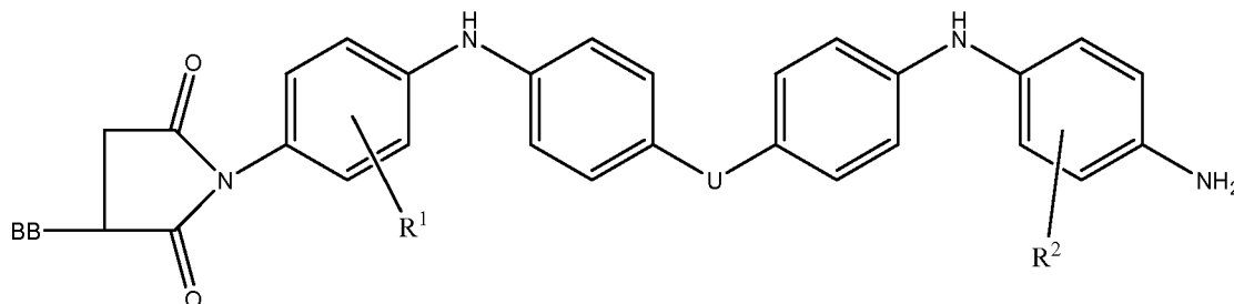
Formula (4)
