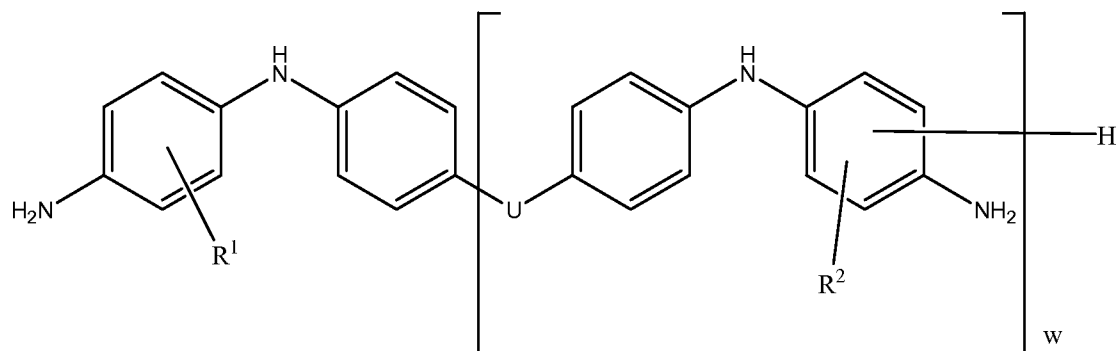
Formula (1a)
