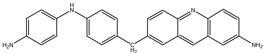
Formula (2a)
