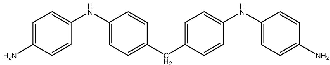
Formula (2)
