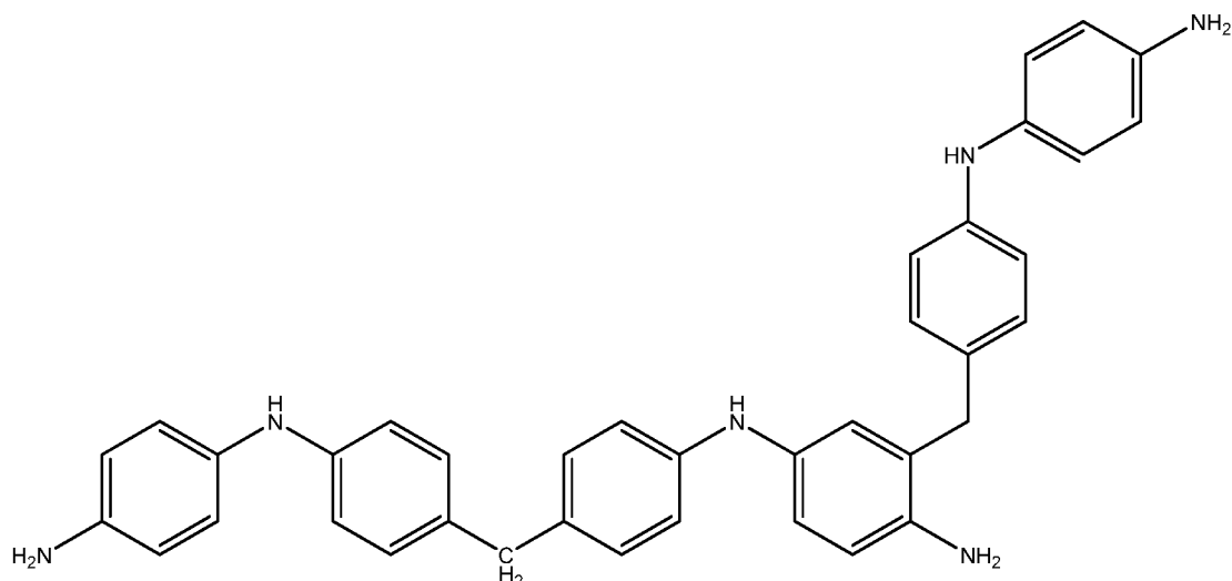
Formula (3)
