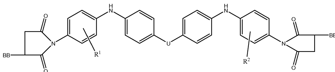
Formula (5)
