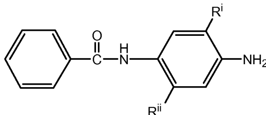
Formula (7)
