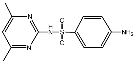
Formula (14)
