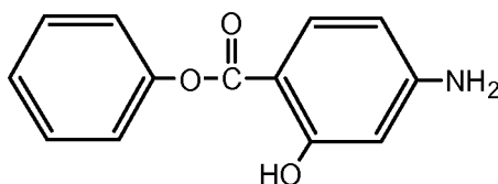
Formula (11)
