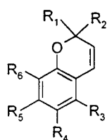
Benzopyrans
