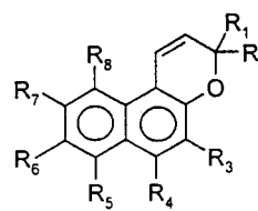
3H-Naphthopyrans
