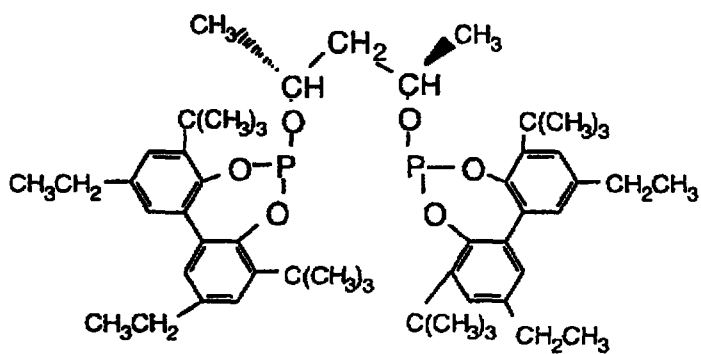
(2R,4R)-di[2,2'-(3,3'-di-tert-butyl-5,5'-diethyl-1,1'-biphenyl)]-2,4-pentylidiphosphite having the formula:
