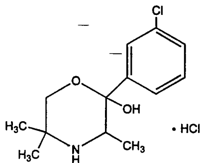
Morpholinol Metabolite of Bupropion HCl
