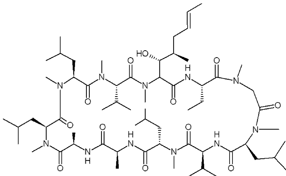
Cyclosporine A
