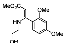
( Z )-Methyl 3-(2,4-dimethoxyphenyl)-3-((2-hydroxyethyl)amino)acrylate
