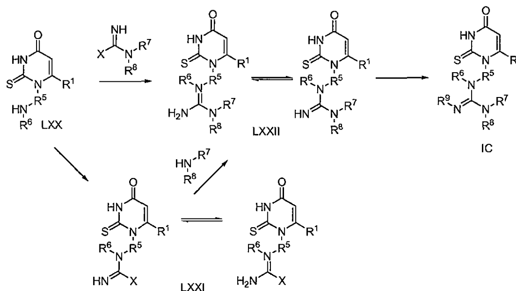
SCHEME IV
