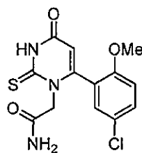
2-(6-(5-Chloro-2-methoxyphenyl)-4-oxo-2-thioxo-3,4-dihydropyrimidin-1(2H)-yl) acetamide
