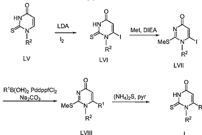
SCHEME II
