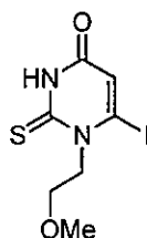
6-Iodo-1-(2-methoxyethyl)-2-thioxo-2,3-dihydropyrimidin-4(1H)-one
