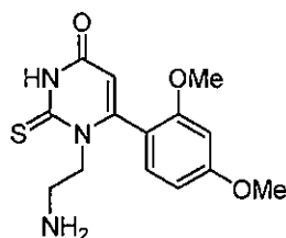
1-(2-aminoethyl)-6-(2,4-dimethoxyphenyl)-2-thioxo-2,3-dihydropyrimidin-4(1H)-one hydrochloride
