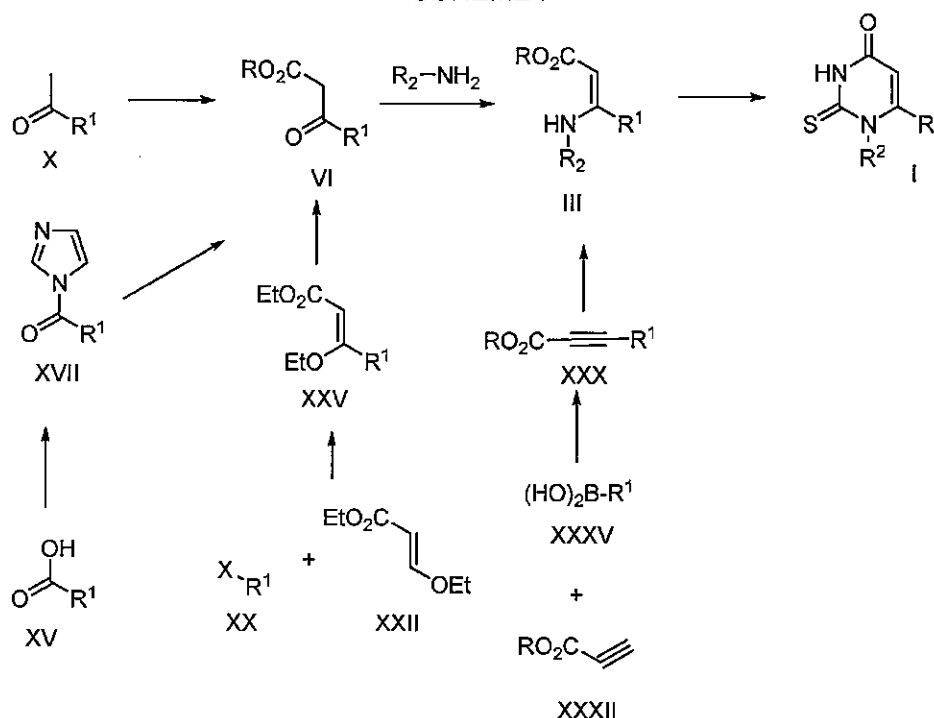
SCHEME I
