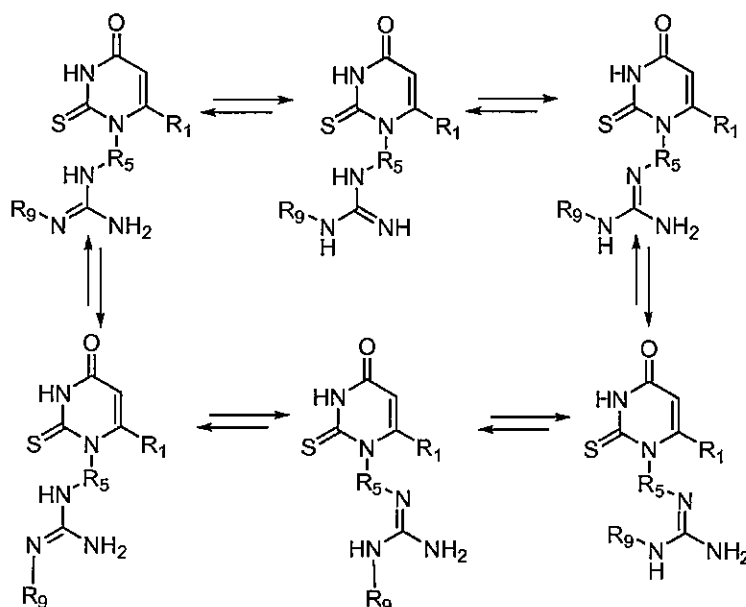
Example of guanidine tautomers and geometric isomers
