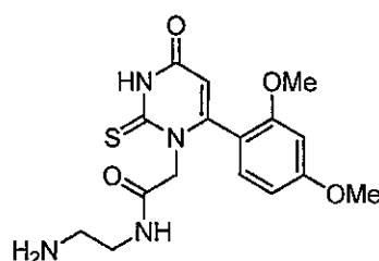
N -(2-aminoethyl)-2-(6-(2,4-dimethoxyphenyl)-4-oxo-2-thioxo-3,4-dihydropyrimidin-1(2H)-yl)acetamide hydrochloride
