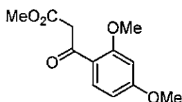
Methyl 3-(2,4-dimethoxyphenyl)-3-oxopropanoate
