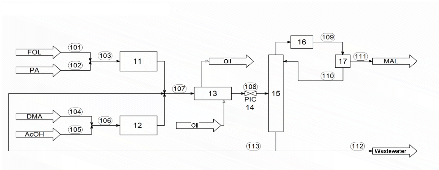
Fig. 2: Possible process flow diagram for step A)
