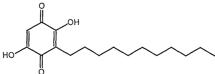
Structure # 1 :- 2,5-Dihydroxy-3-undecyl-p-benzoquinone (embelin)
