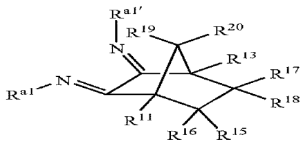
Structure 6f
