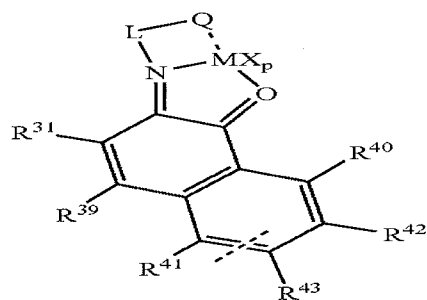
Structure 23d
