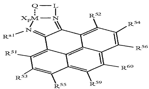
Structure 26e
