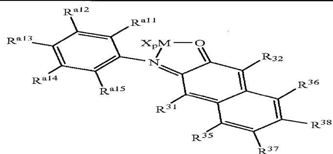
Structure 34d
