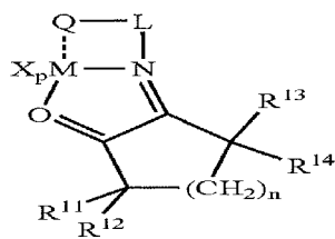
Structure 15d
