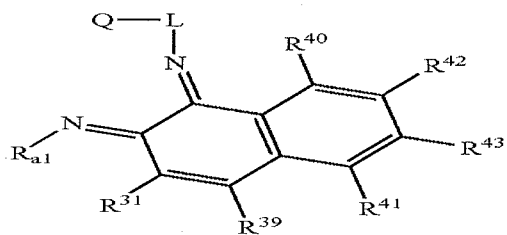
Structure 22f
