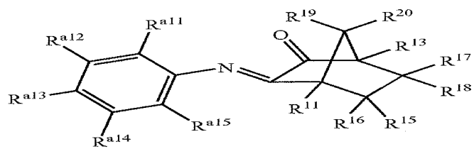
Structure 32b
