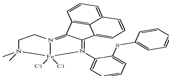
Structure XVI
