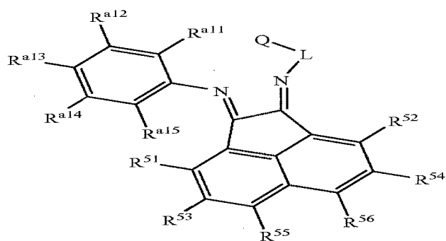
Structure 37f
