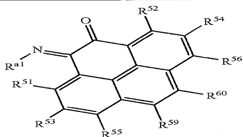
Structure 13b
