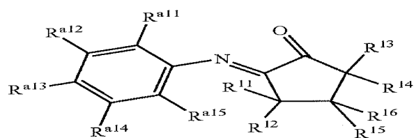
Structure 30b
