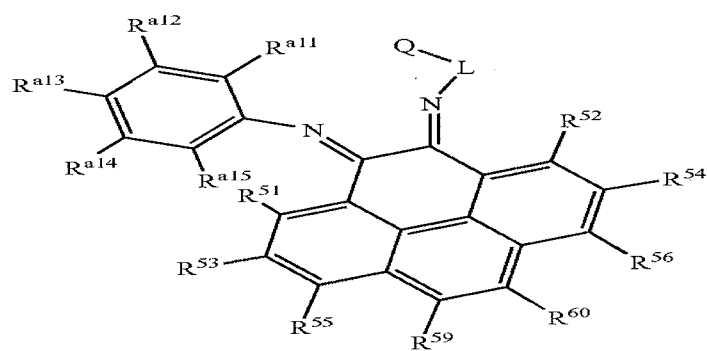
Structure 39f
