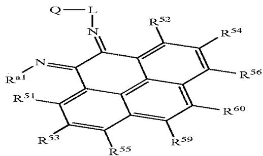
Structure 26f
