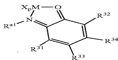
Structure 7d
