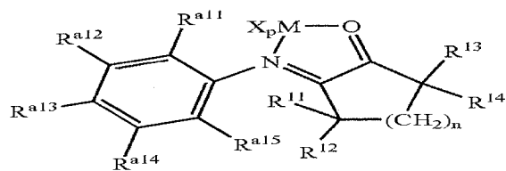
Structure 28d
