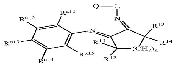
Structure 28f
