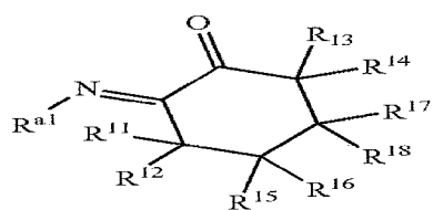
Structure 5b
