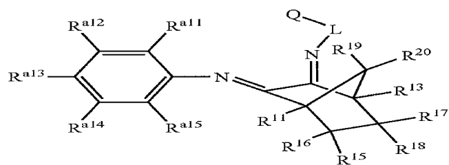
Structure 32f
