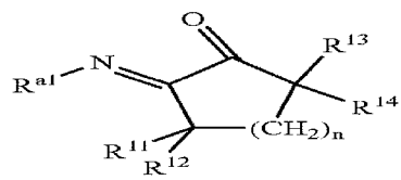
Structure 2b
