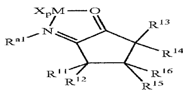
Structure 4d
