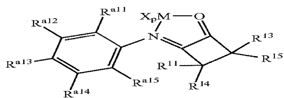
Structure 29d
