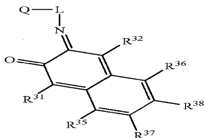
Structure 21b
