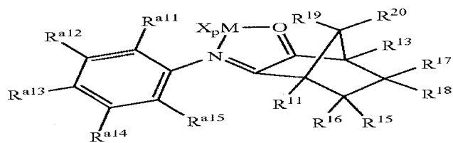
Structure 32d
