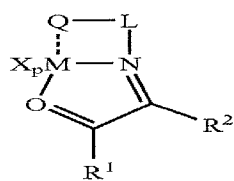
Structure 14d
