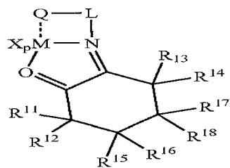
Structure 18d
