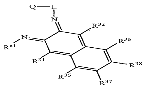
Structure 21f
