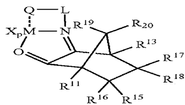
Structure 19d
