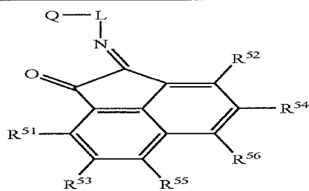
Structure 24b
