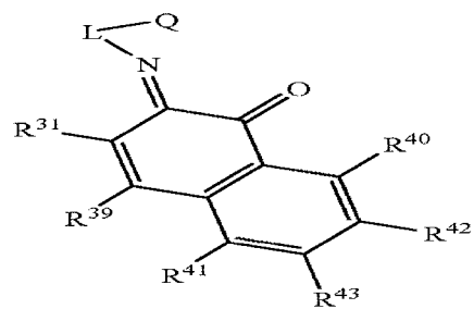
Structure 23b
