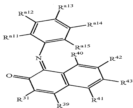
Structure 36b
