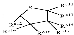
Structure 12c
