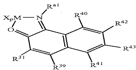
Structure 10d
