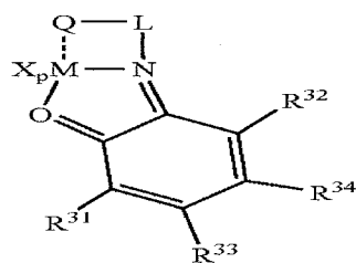
Structure 20d
