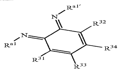
Structure 7f
