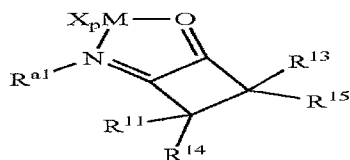
Structure 3d
