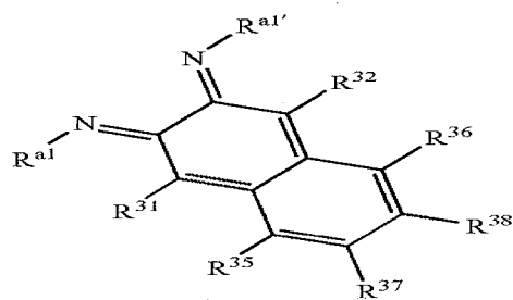
Structure 8f
