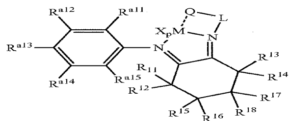
Structure 31e
