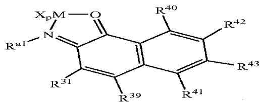
Structure 9d
