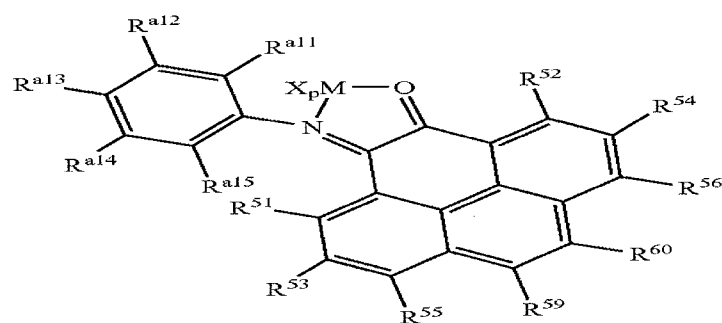
Structure 39d
