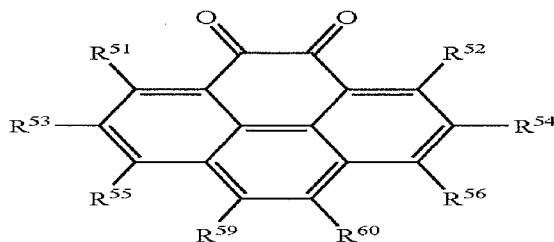
Structure 12
