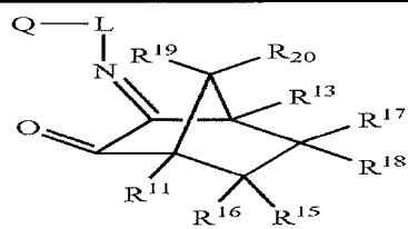
Structure 19b
