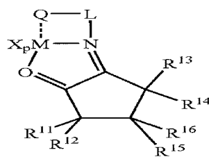
Structure 17d
