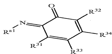
Structure 7b
