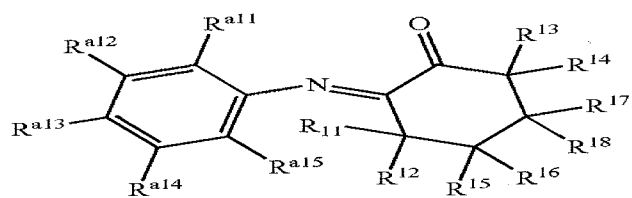
Structure 31b
