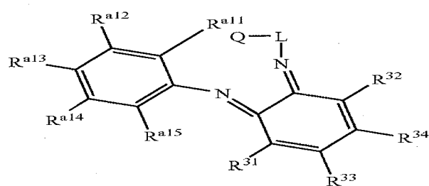
Structure 33f
