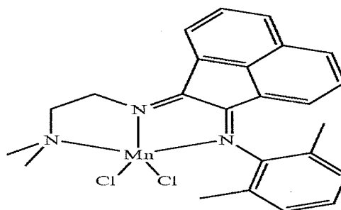
Structure XXII
