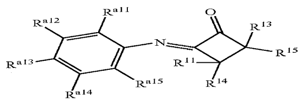
Structure 29b
