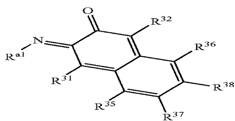
Structure 8b
