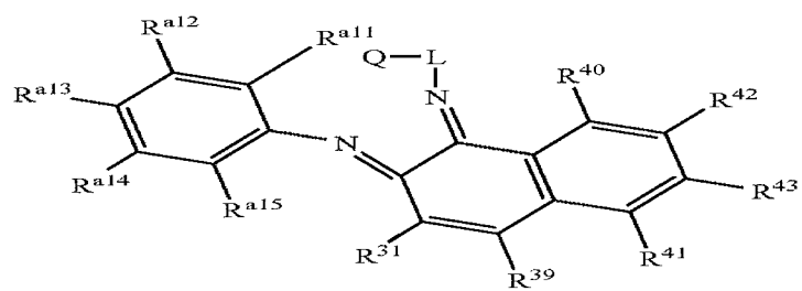
Structure 35f
