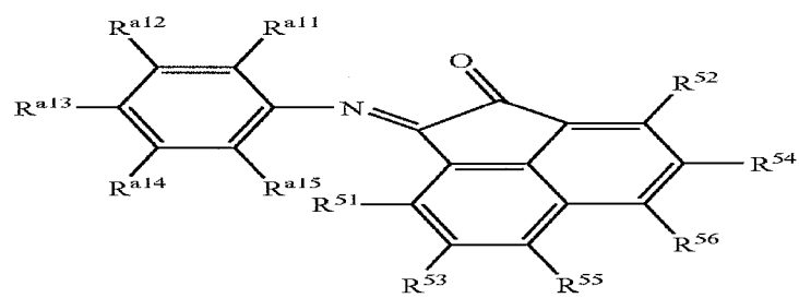
Structure 37b
