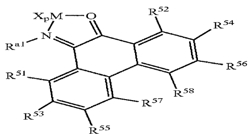
Structure 12d
