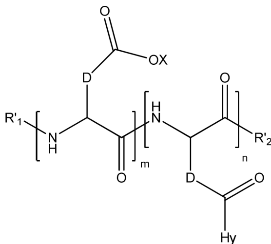
Formula VIIa
