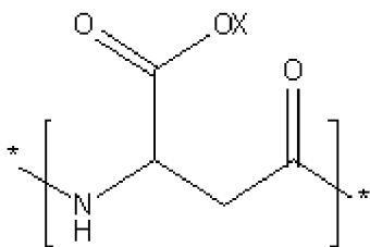
Formula VIII
