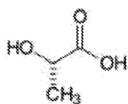
L-(+)-Lactic acid
