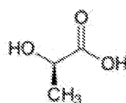
D-(-)-Lactic acid
